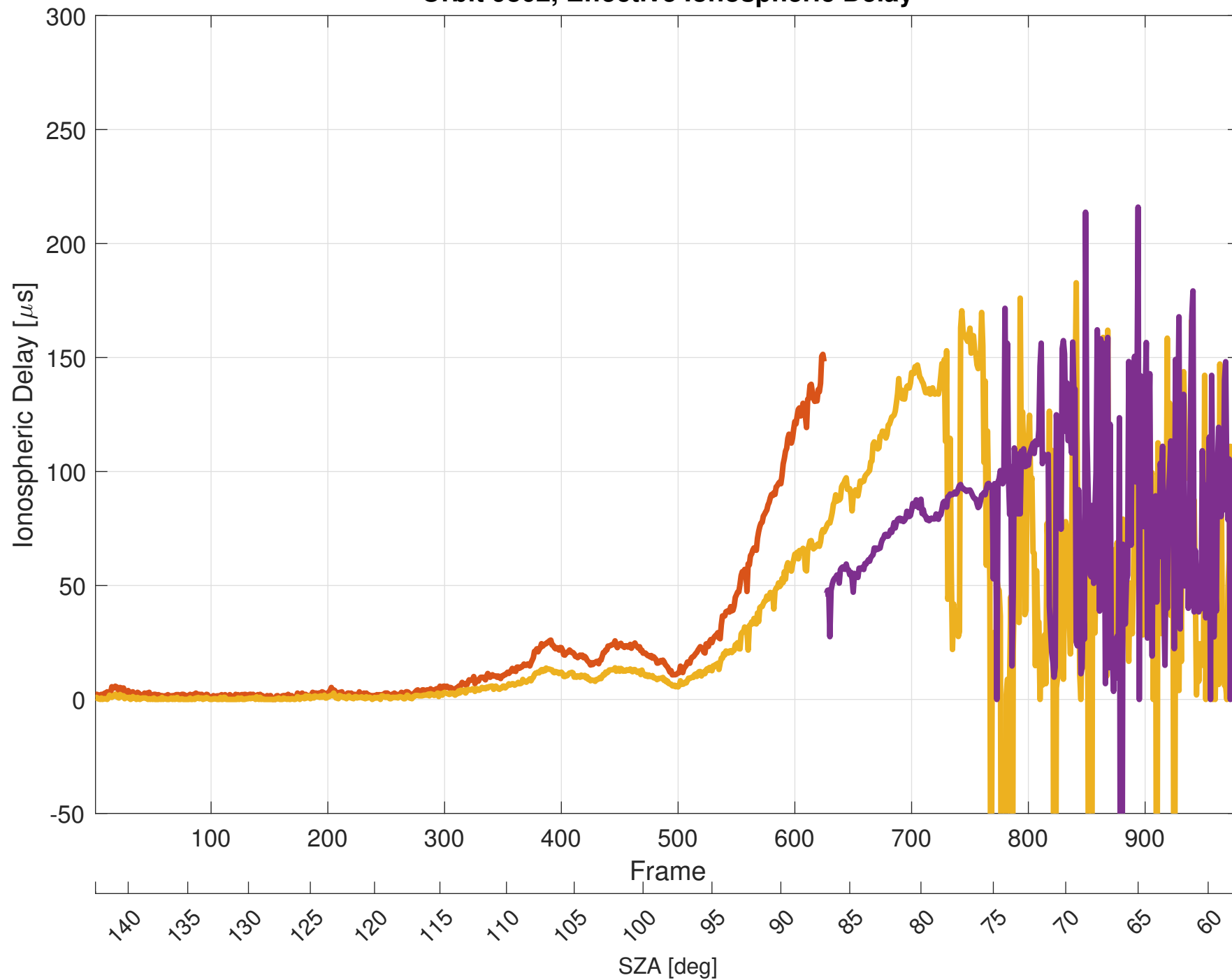
Orbit 9802, Effective Ionospheric Delay
