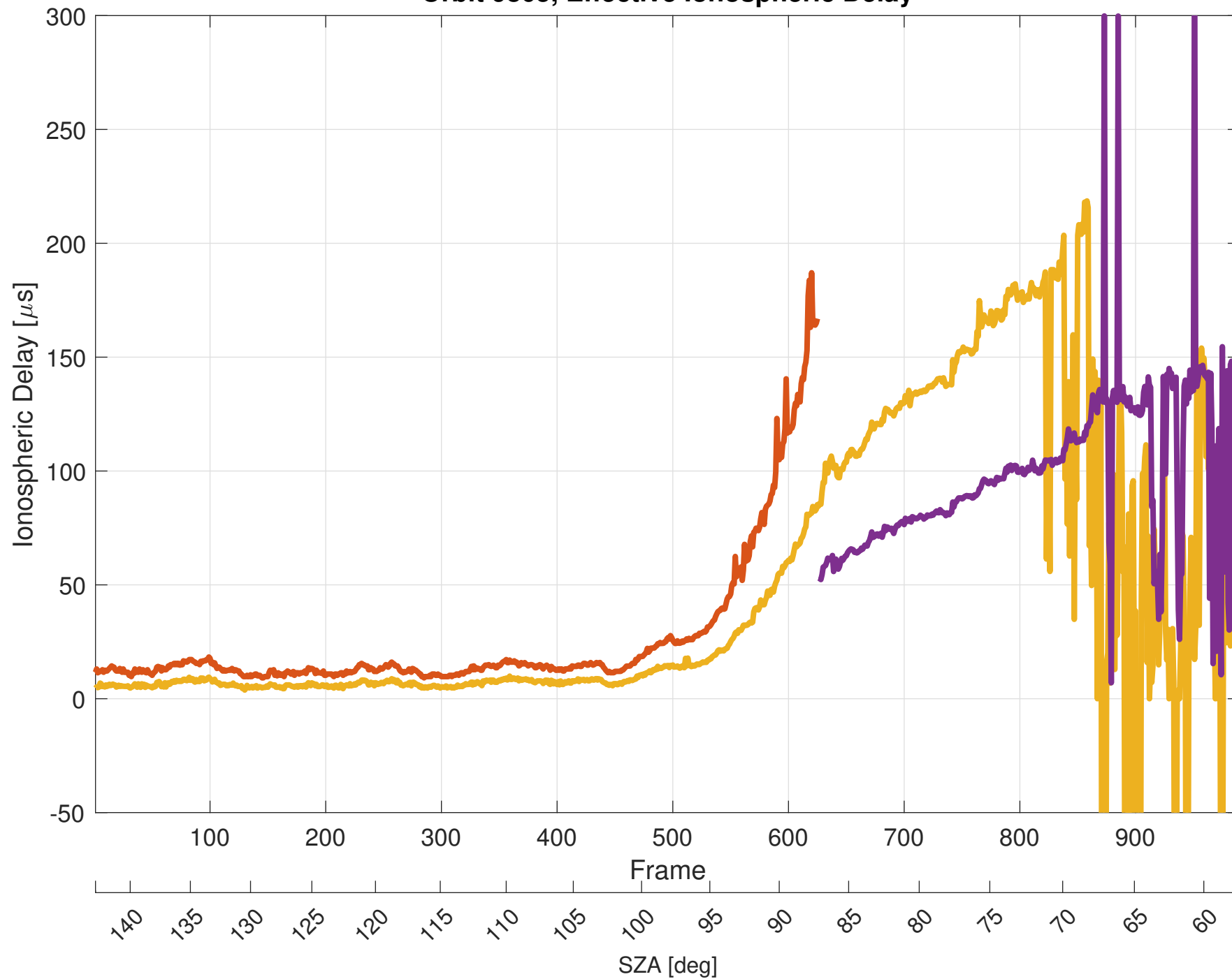
Orbit 9805, Effective Ionospheric Delay
