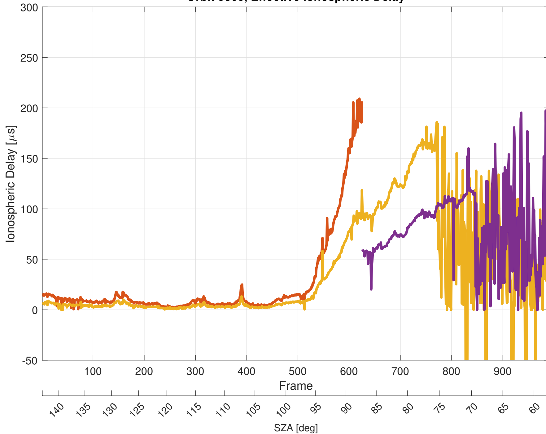
Orbit 9806, Effective Ionospheric Delay
