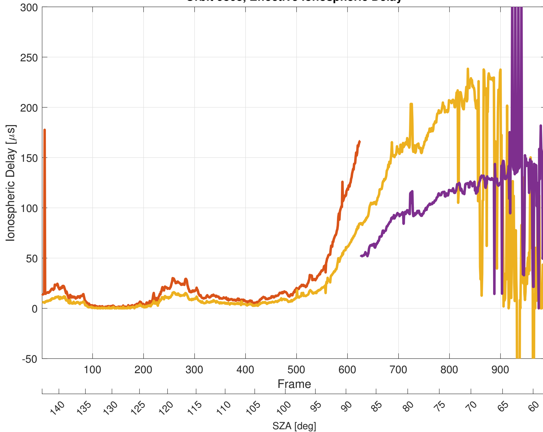
Orbit 9808, Effective Ionospheric Delay
