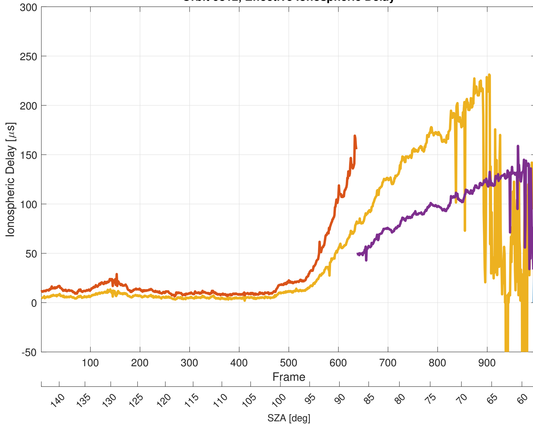
Orbit 9812, Effective Ionospheric Delay
