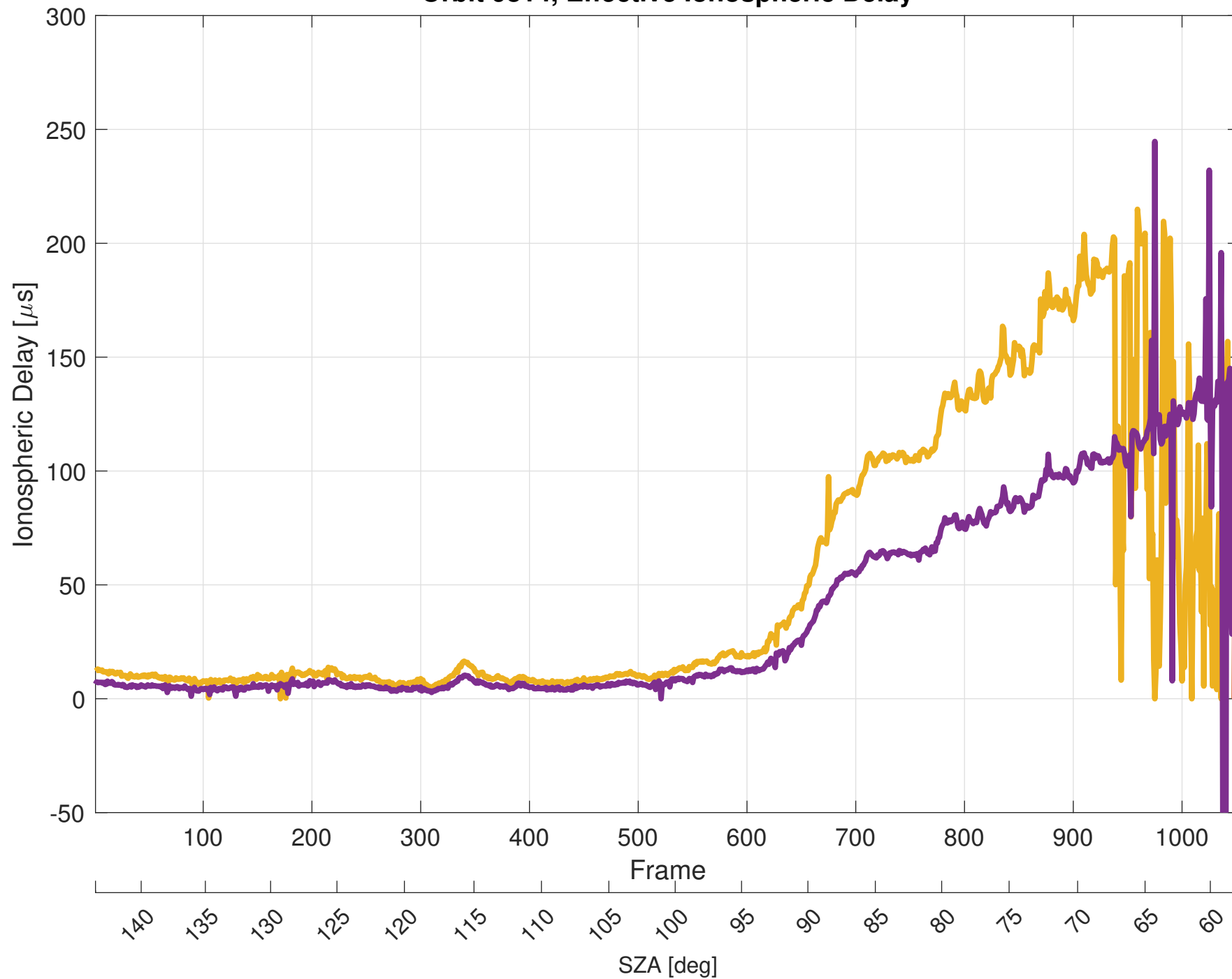
Orbit 9814, Effective Ionospheric Delay
