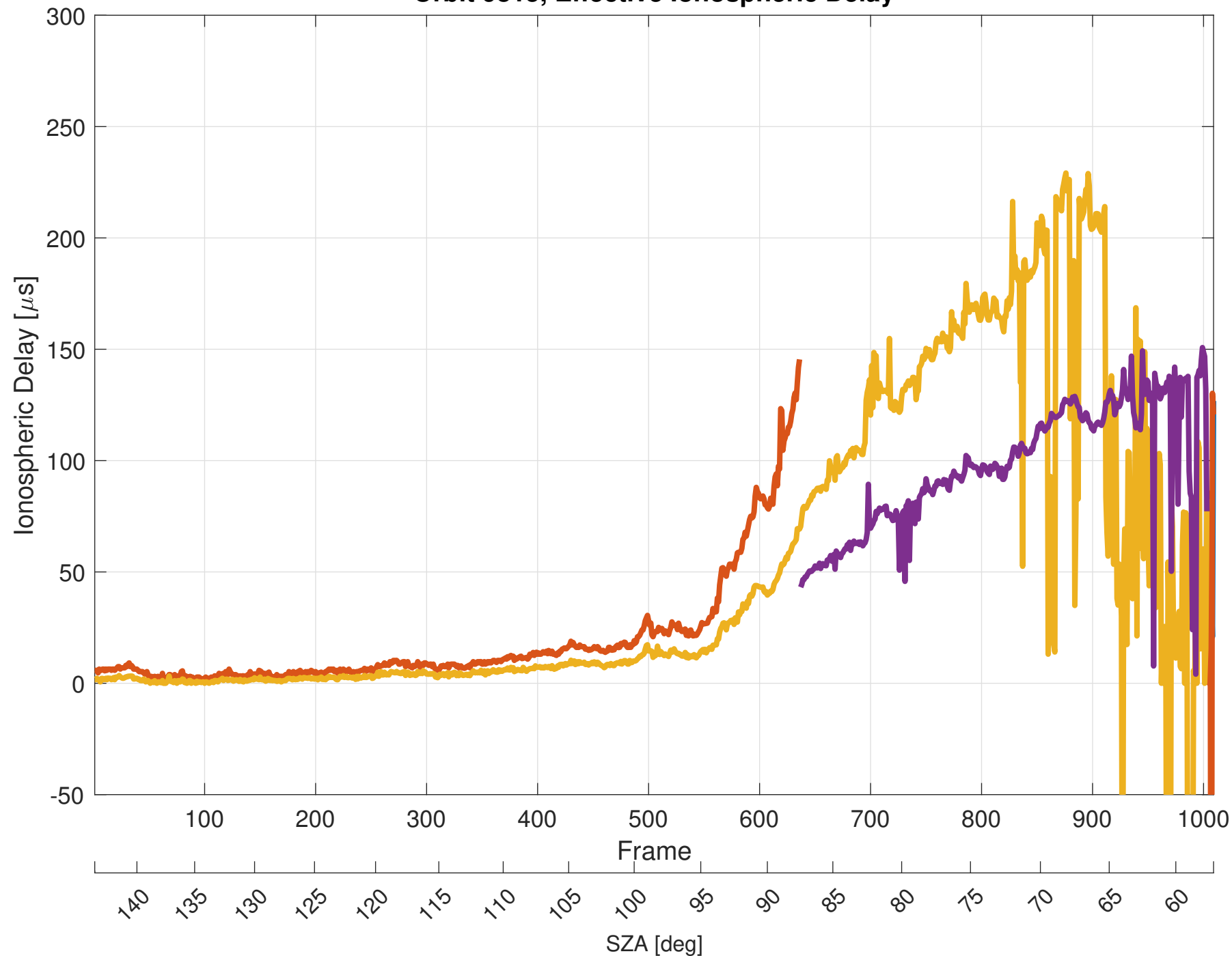
Orbit 9815, Effective Ionospheric Delay
