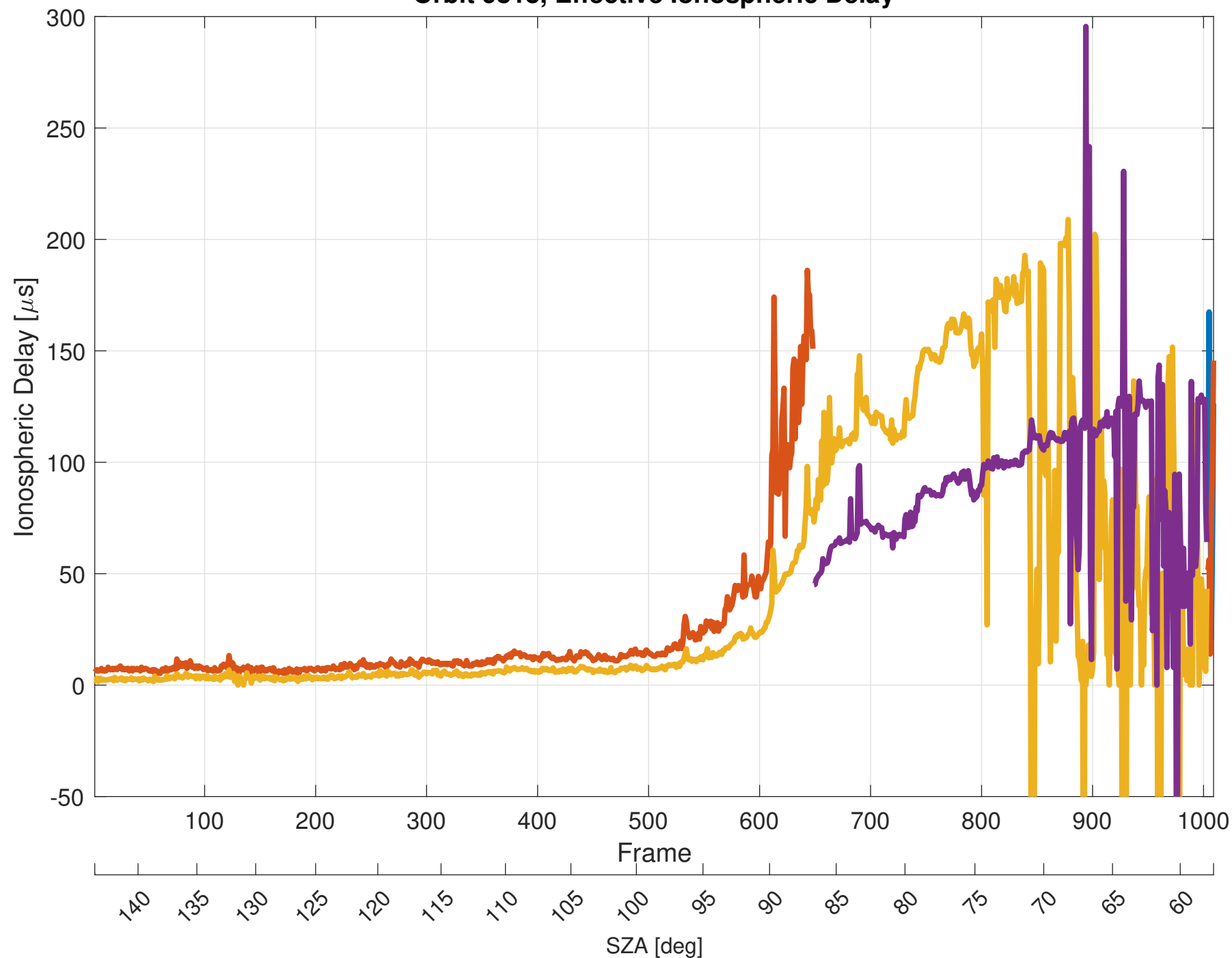
Orbit 9818, Effective Ionospheric Delay
