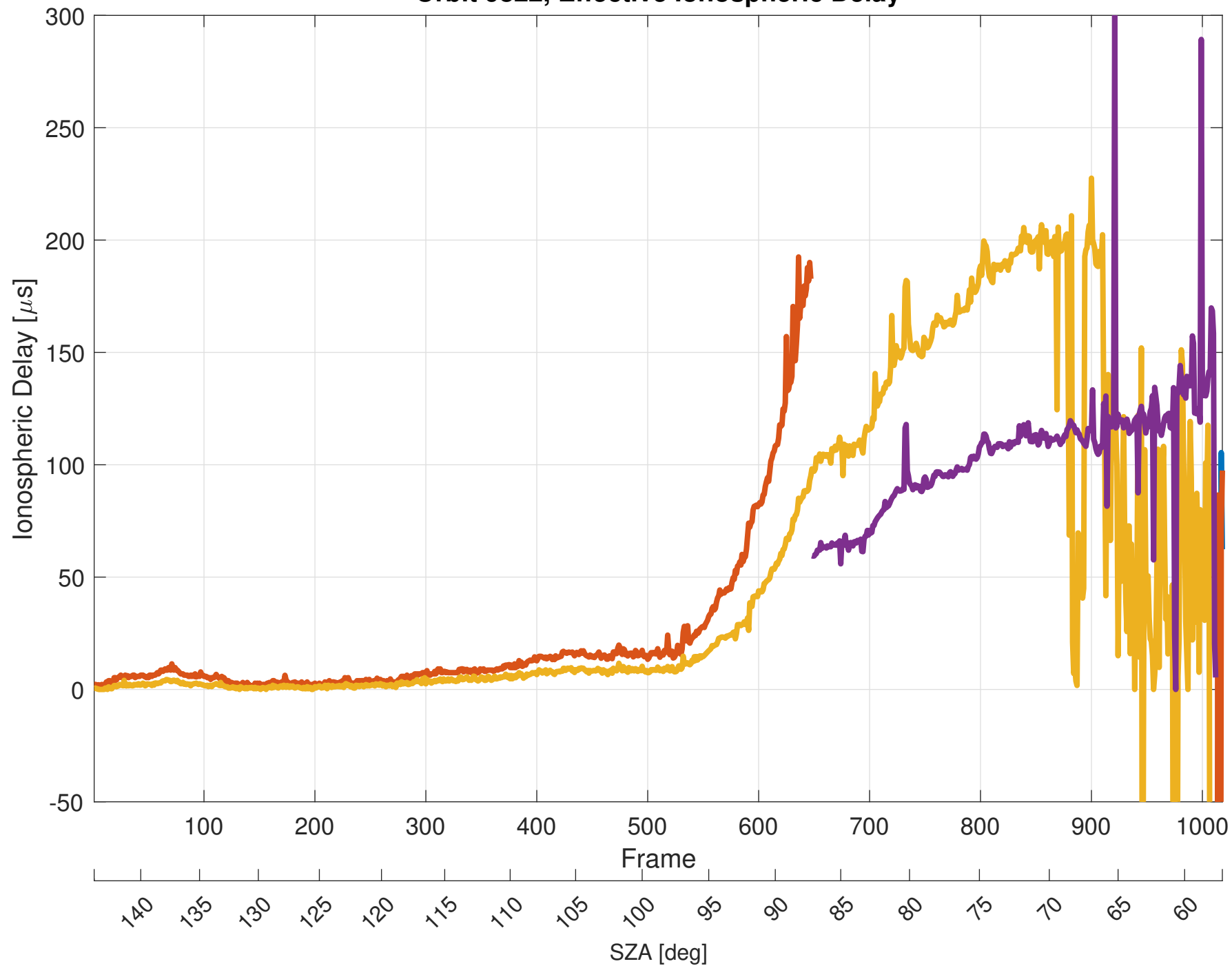
Orbit 9822, Effective Ionospheric Delay
