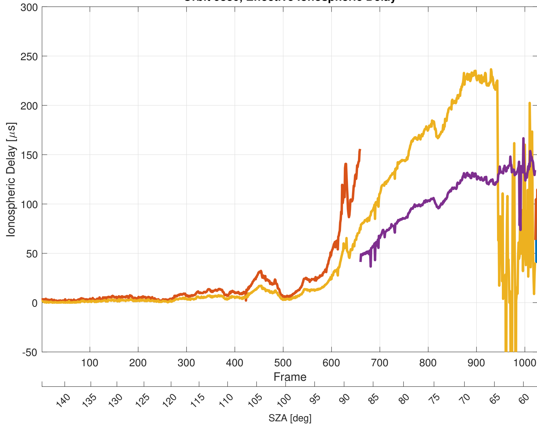
Orbit 9830, Effective Ionospheric Delay
