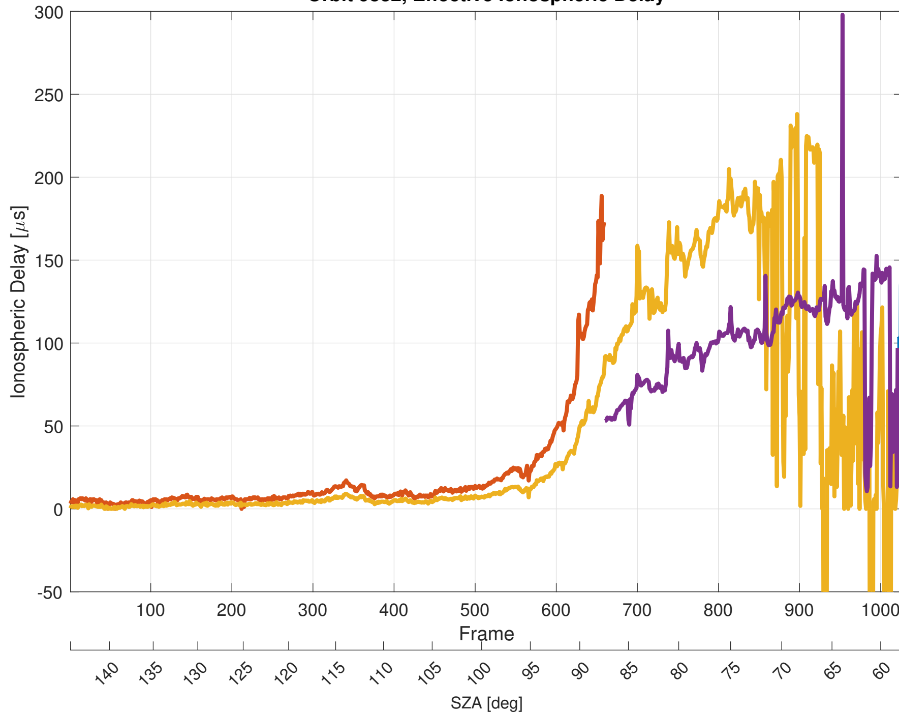
Orbit 9832, Effective Ionospheric Delay
