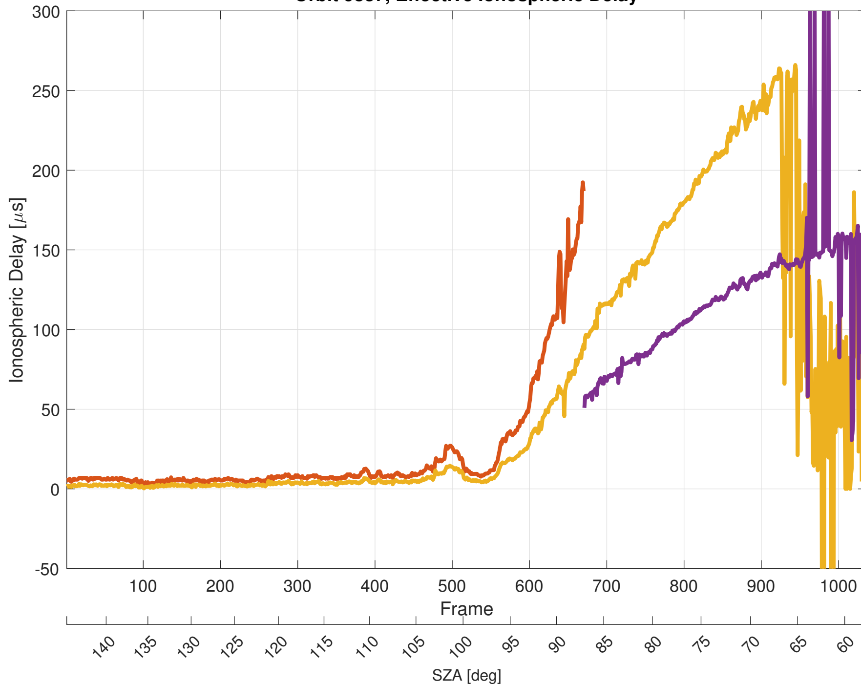
Orbit 9837, Effective Ionospheric Delay
