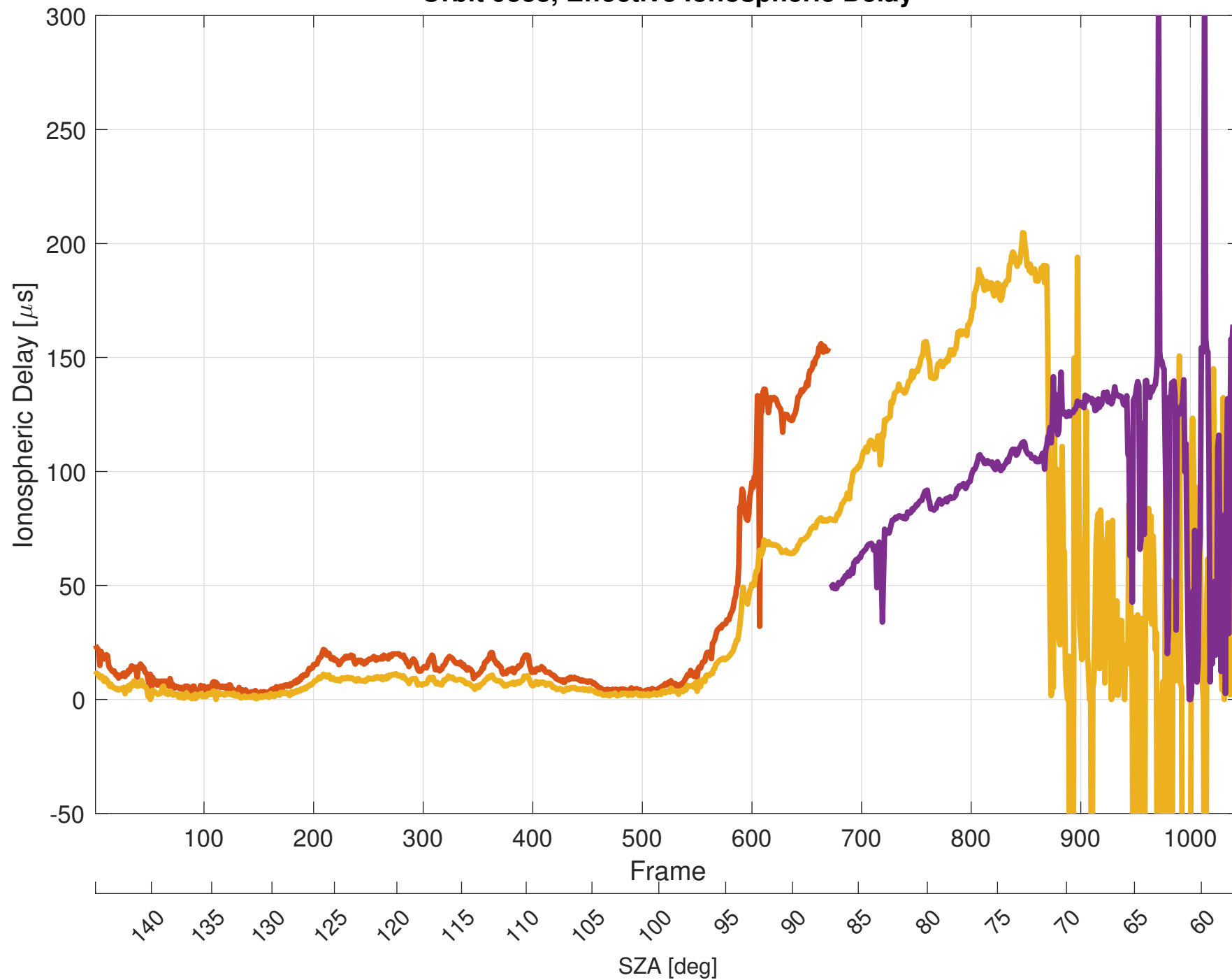
Orbit 9838, Effective Ionospheric Delay
