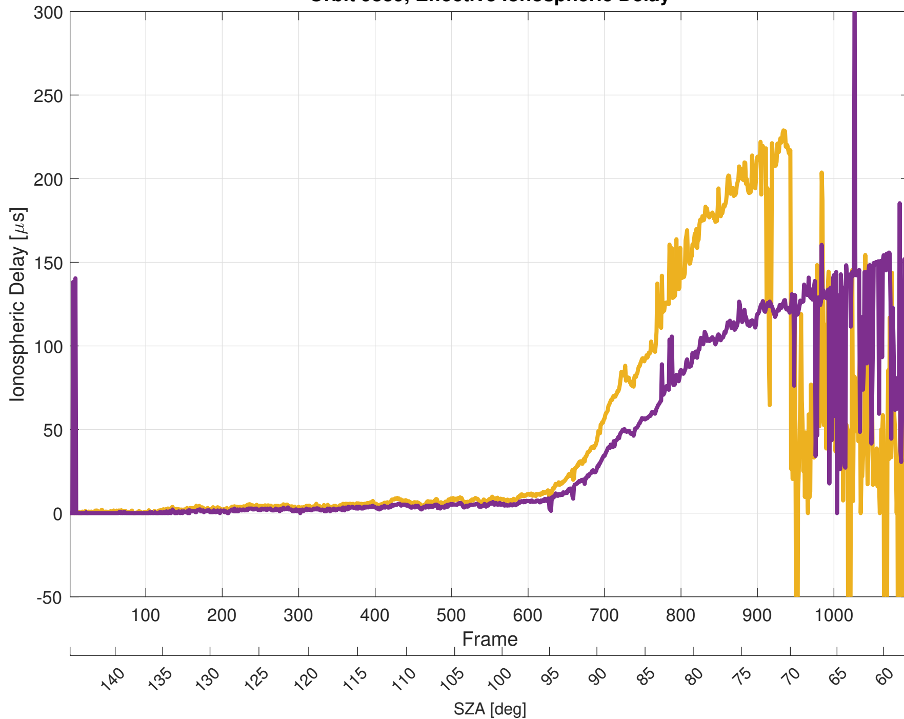
Orbit 9839, Effective Ionospheric Delay
