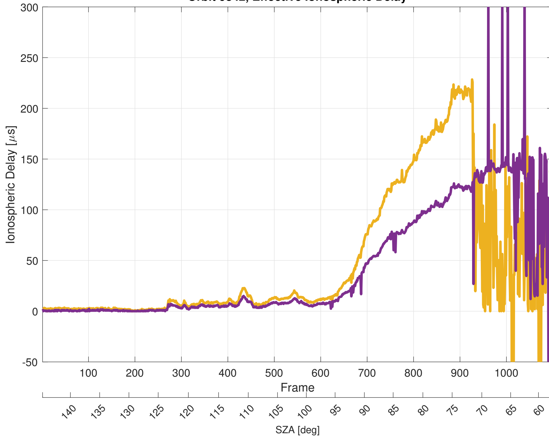
Orbit 9842, Effective Ionospheric Delay
