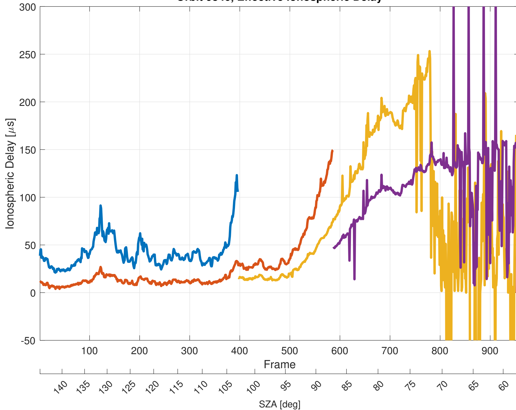
Orbit 9846, Effective Ionospheric Delay
