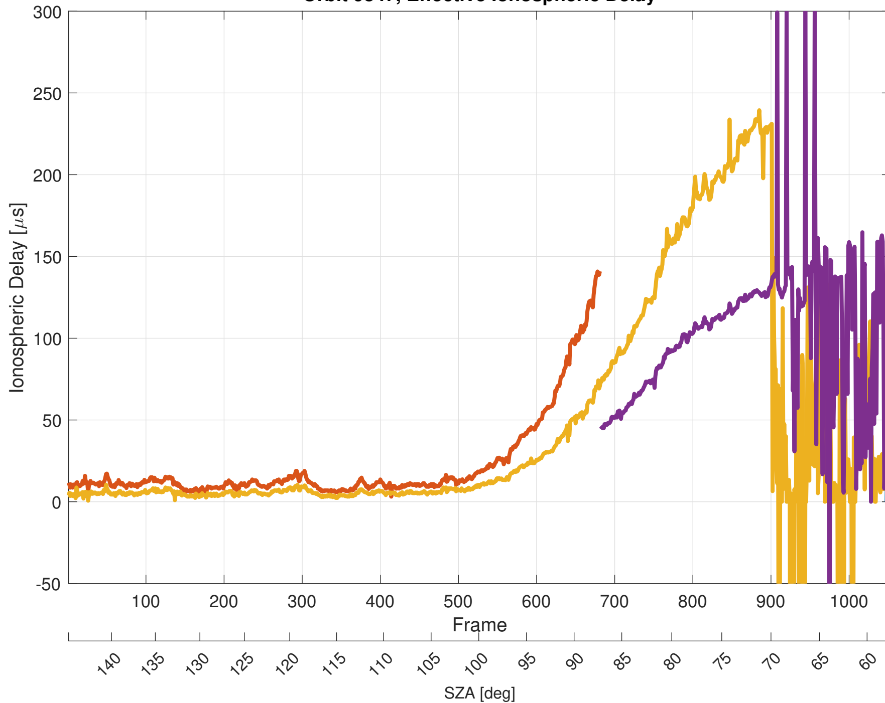
Orbit 9847, Effective Ionospheric Delay
