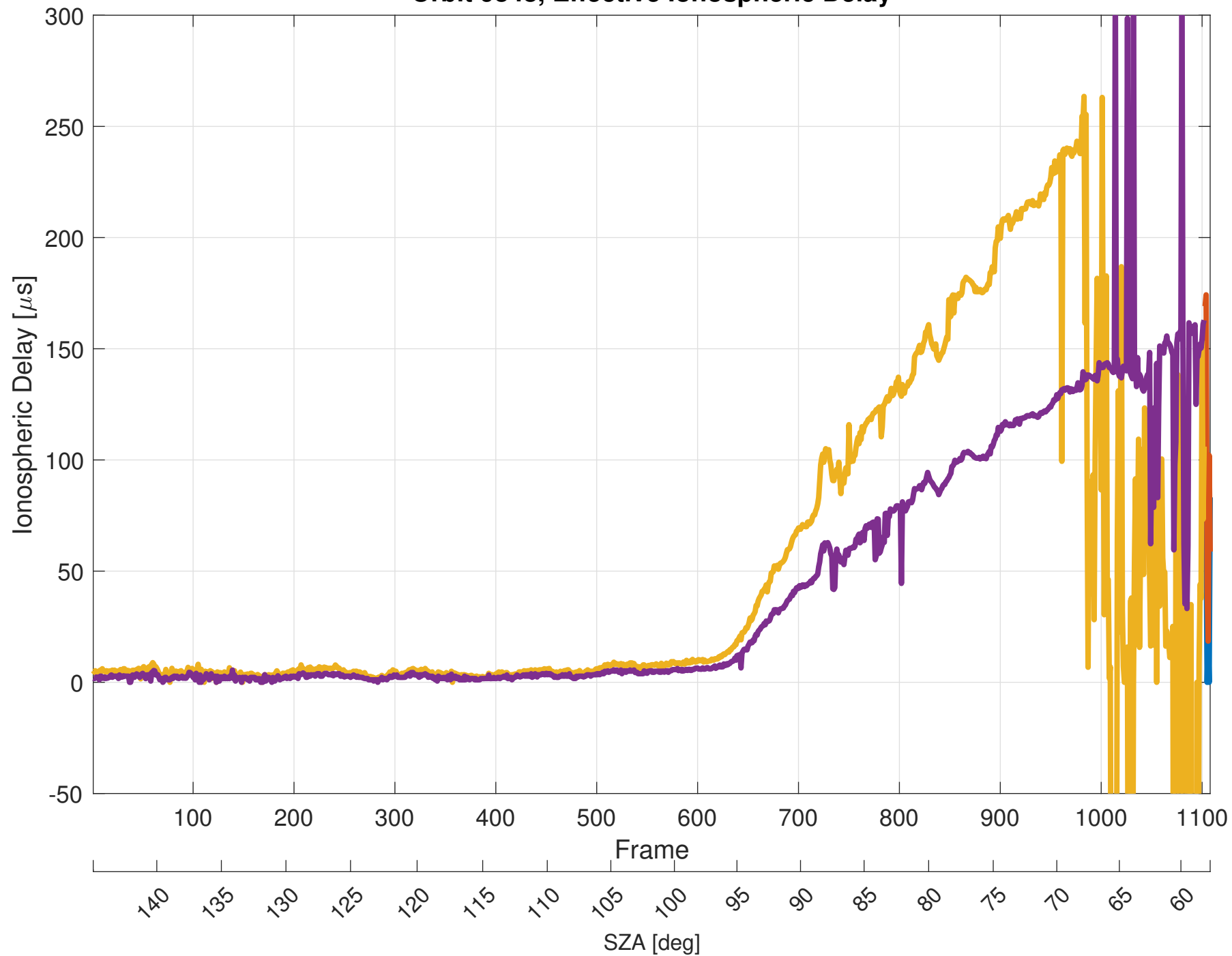
Orbit 9848, Effective Ionospheric Delay
