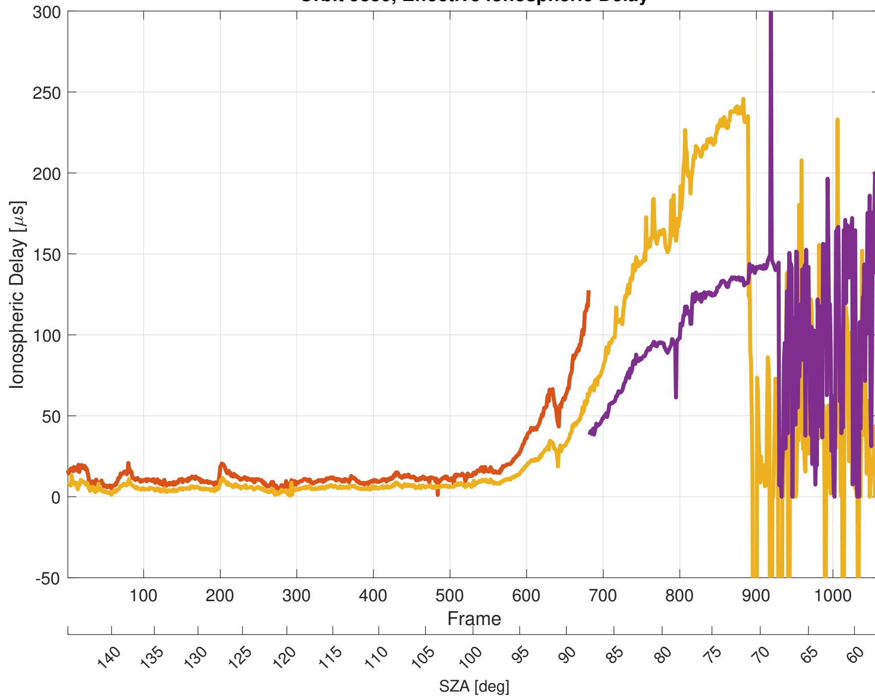
Orbit 9850, Effective Ionospheric Delay
