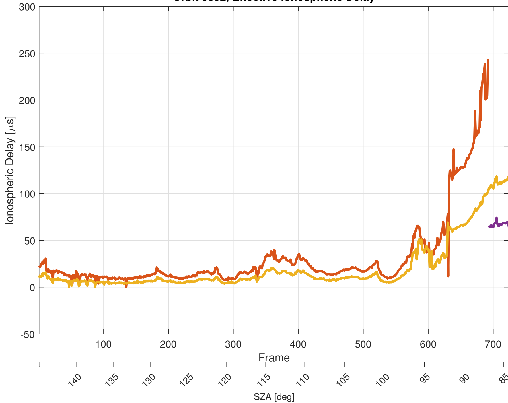
Orbit 9852, Effective Ionospheric Delay
