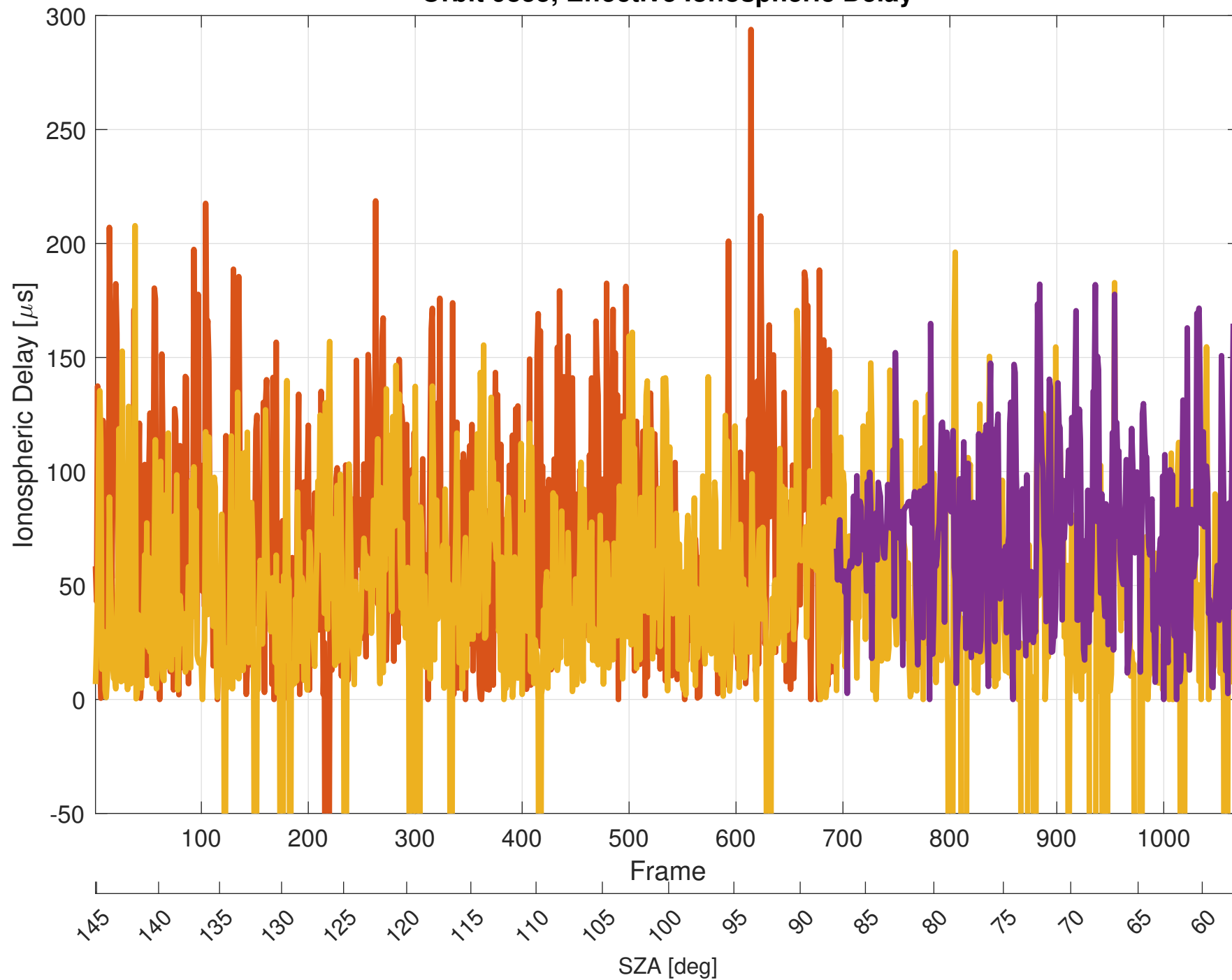
Orbit 9855, Effective Ionospheric Delay
