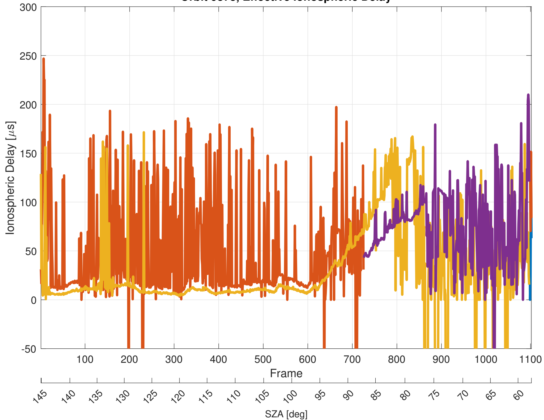
Orbit 9878, Effective Ionospheric Delay
