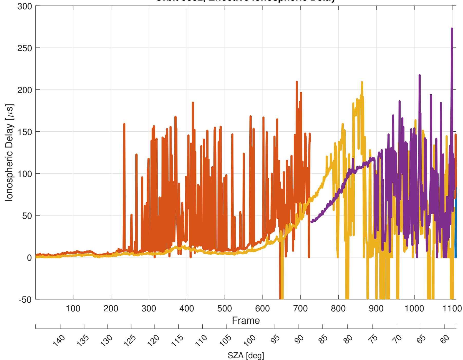
Orbit 9882, Effective Ionospheric Delay
