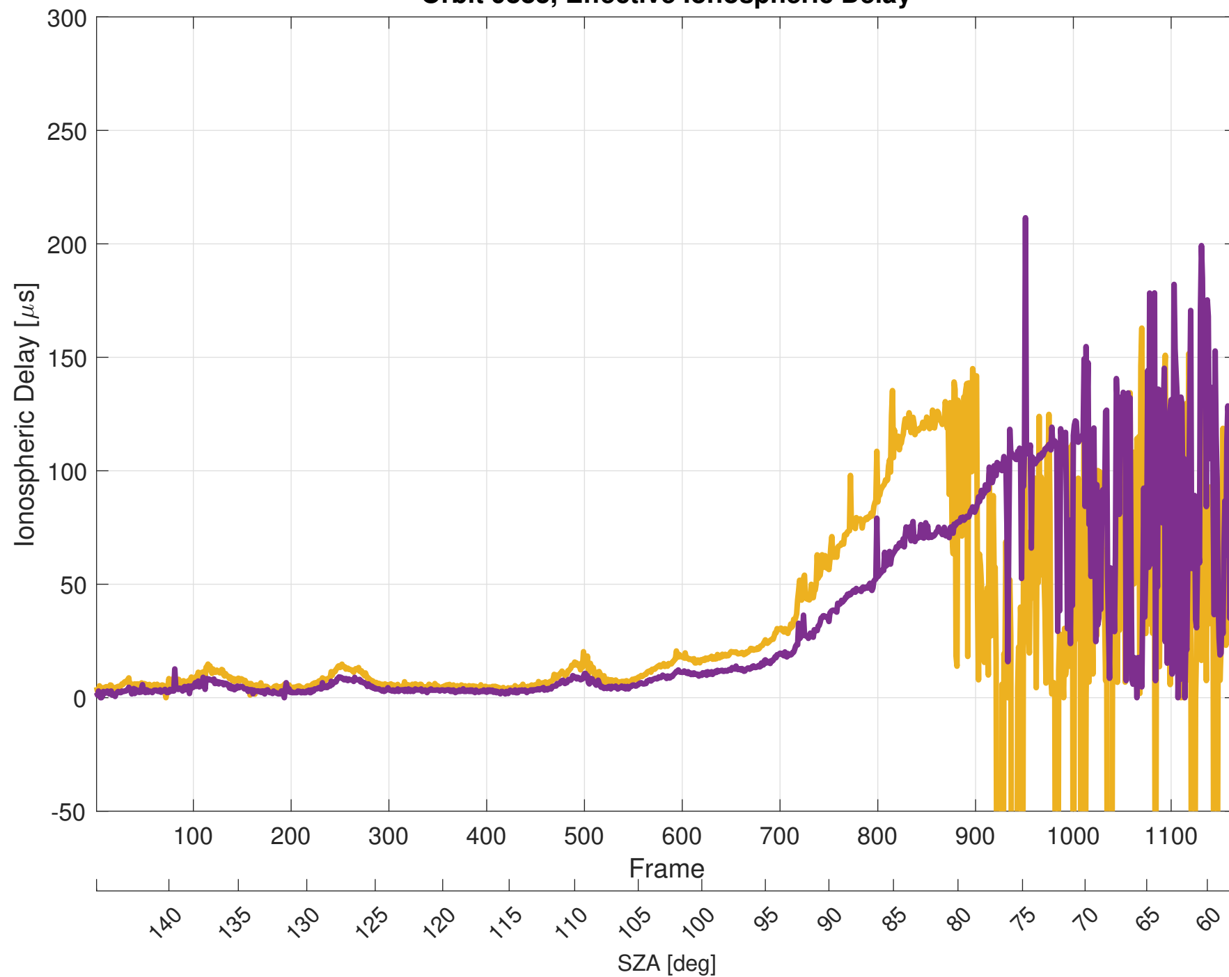
Orbit 9883, Effective Ionospheric Delay
