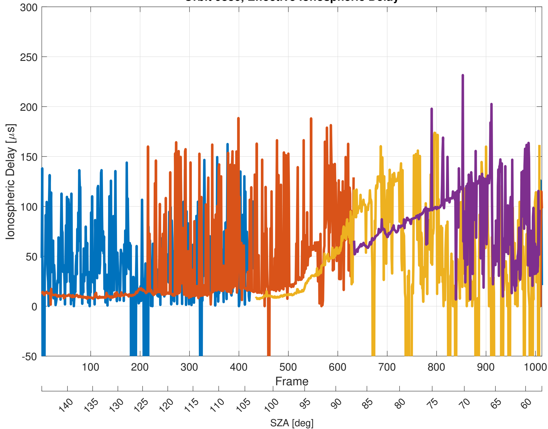
Orbit 9886, Effective Ionospheric Delay
