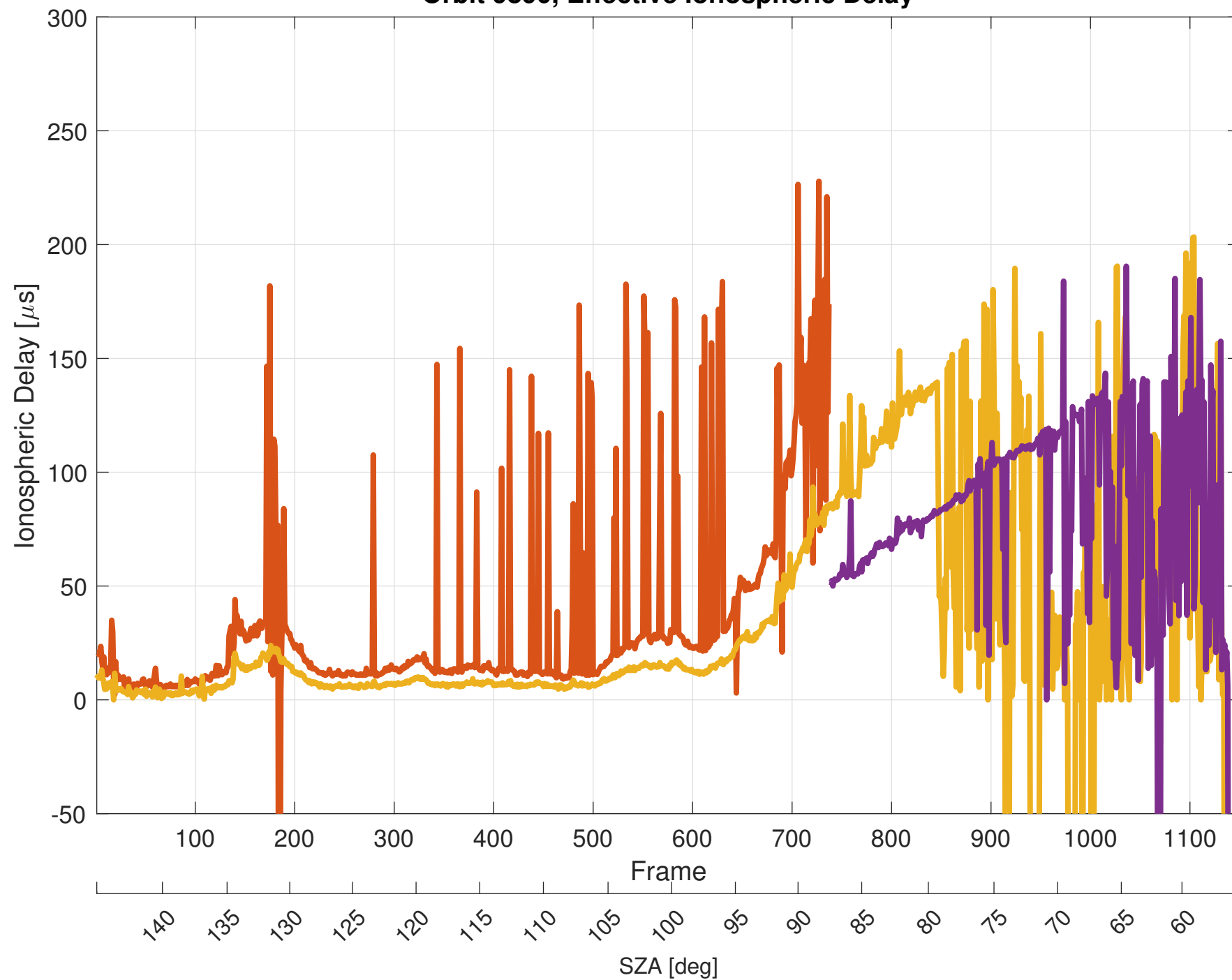
Orbit 9890, Effective Ionospheric Delay
