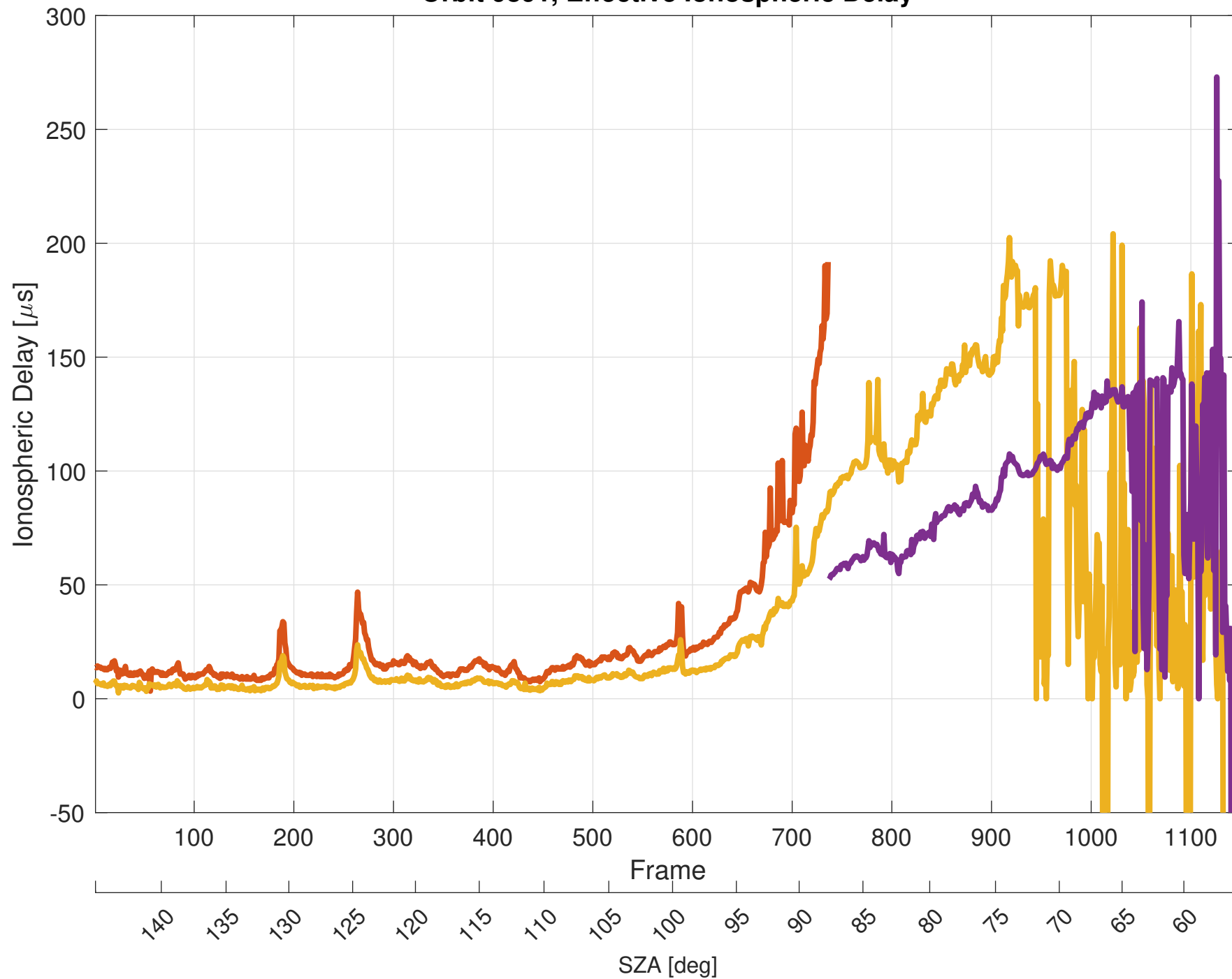
Orbit 9891, Effective Ionospheric Delay
