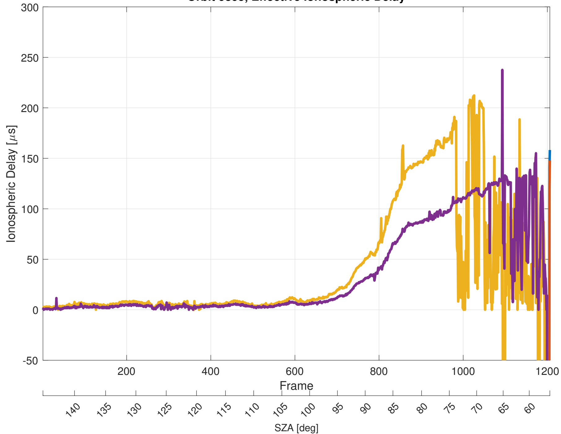
Orbit 9895, Effective Ionospheric Delay
