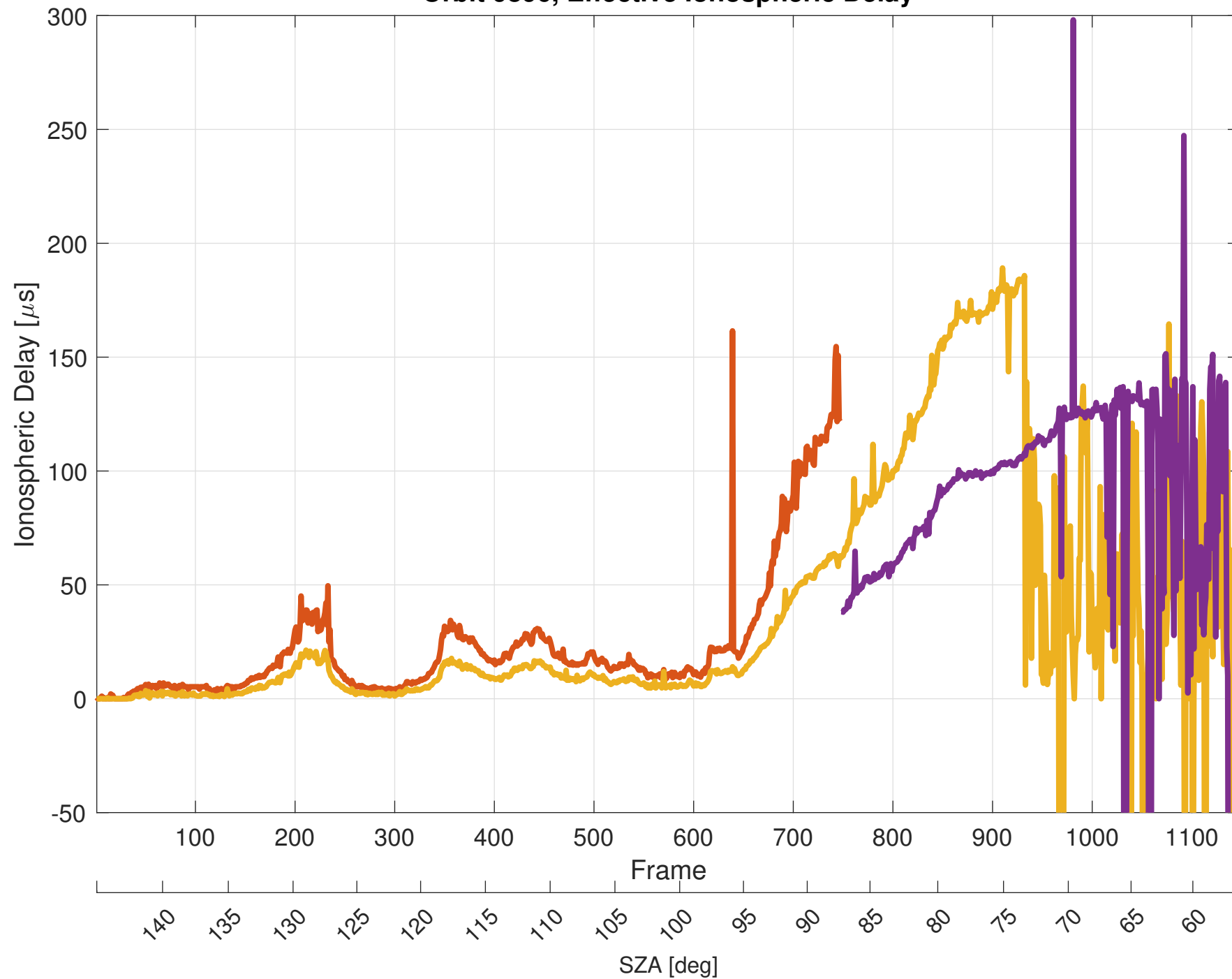
Orbit 9896, Effective Ionospheric Delay
