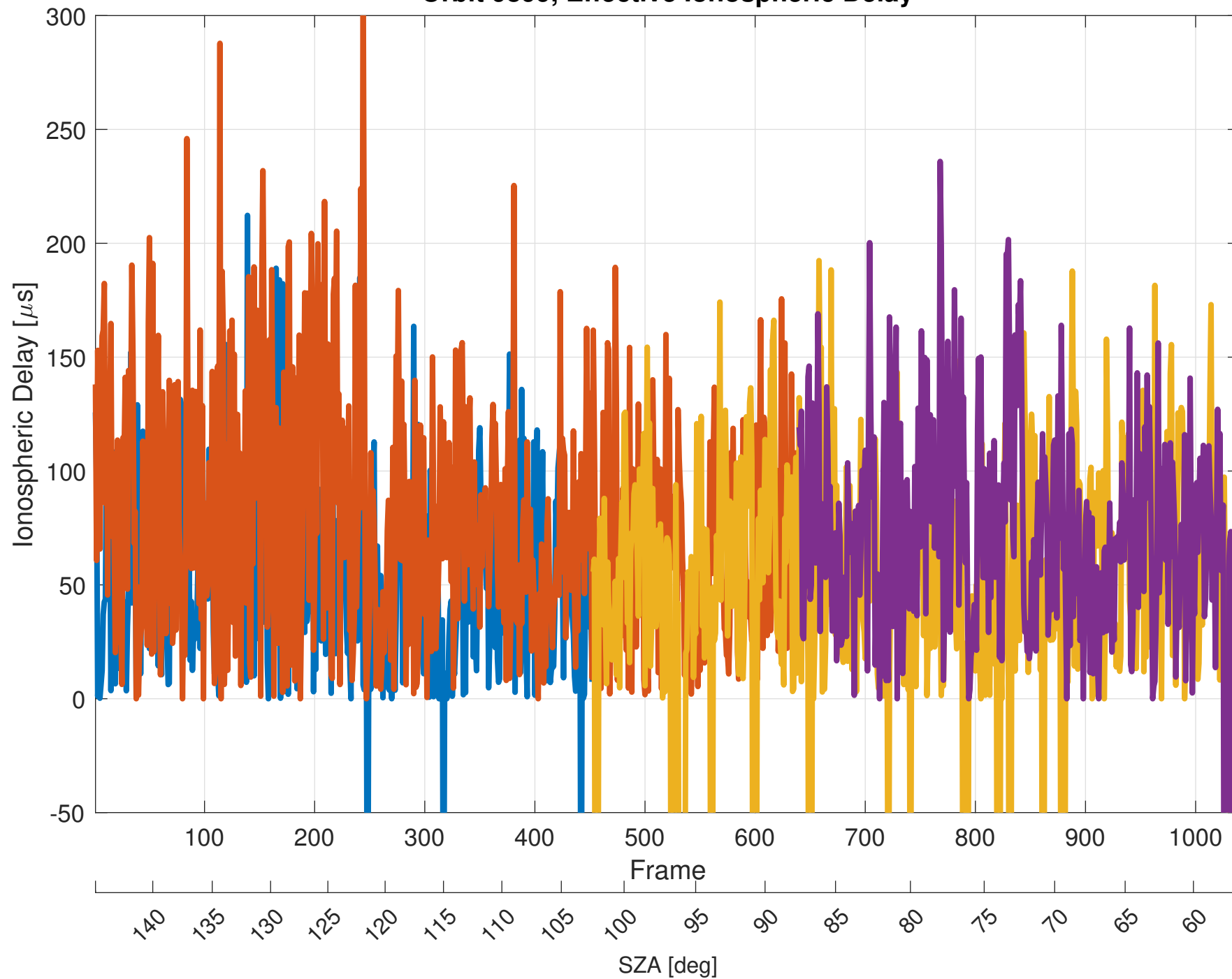
Orbit 9899, Effective Ionospheric Delay
