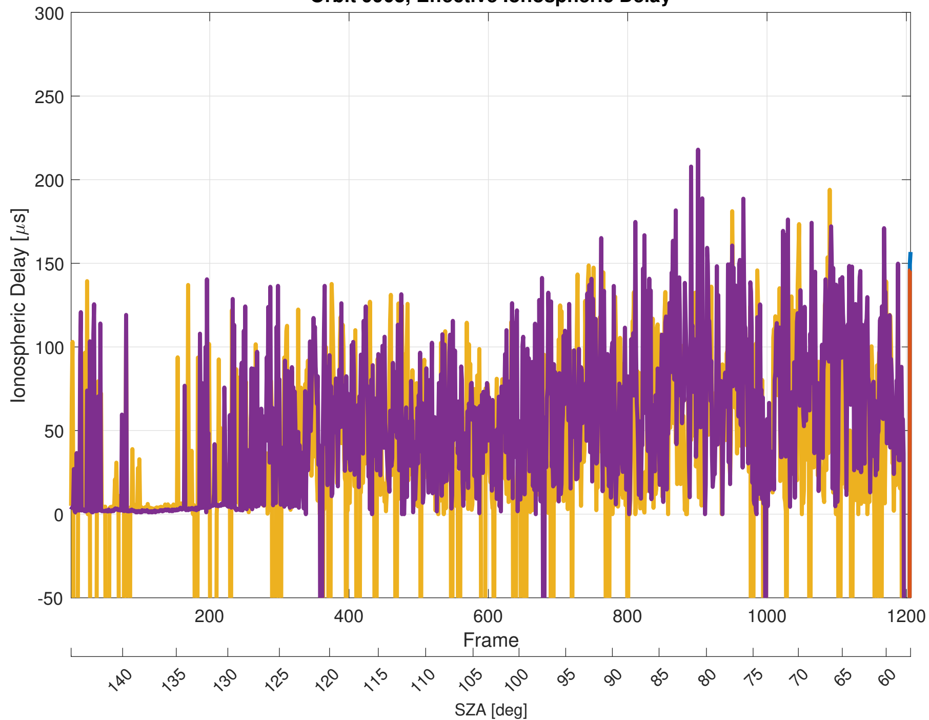
Orbit 9903, Effective Ionospheric Delay
