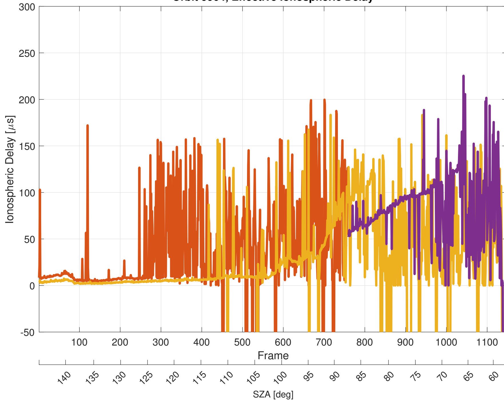
Orbit 9904, Effective Ionospheric Delay
