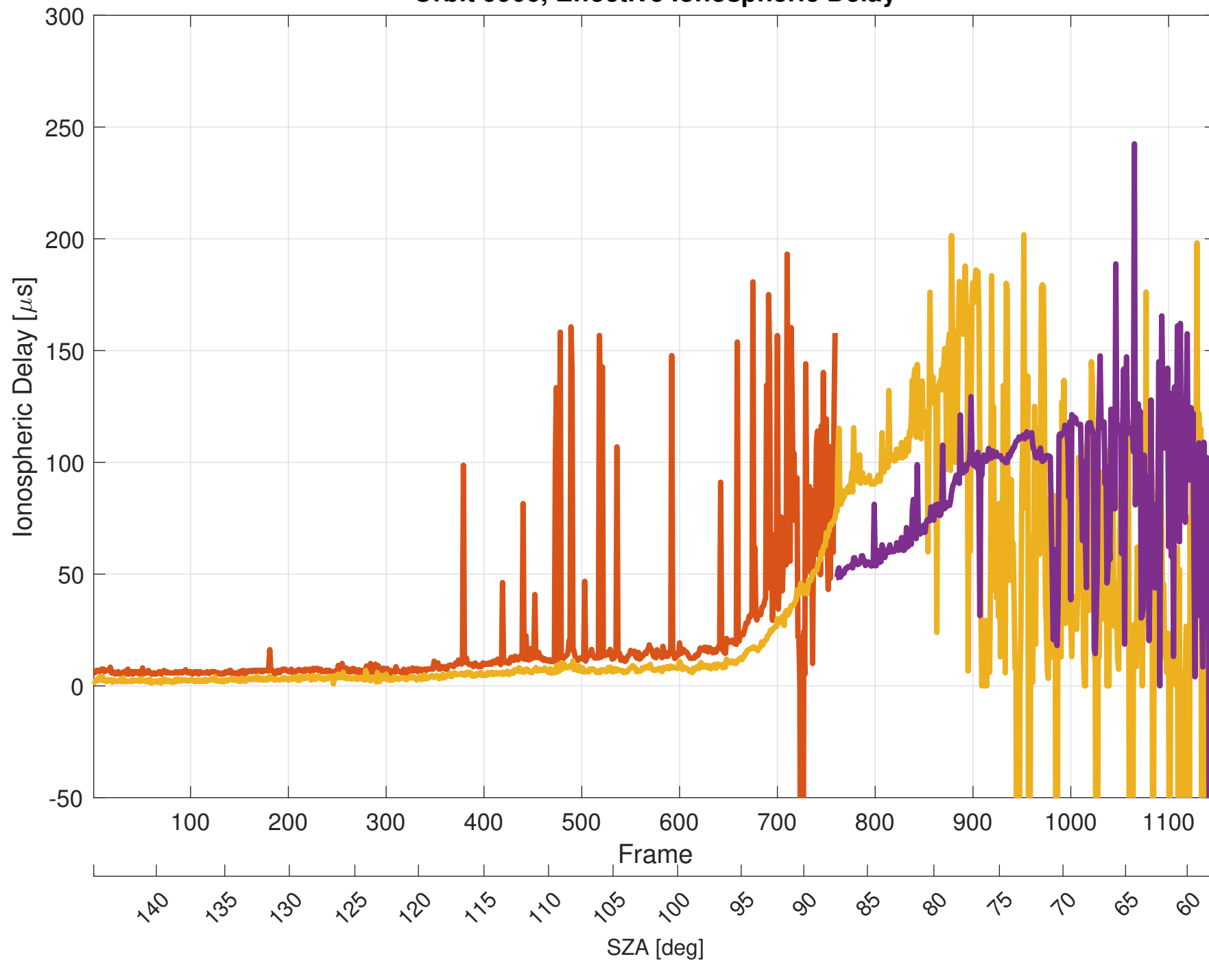
Orbit 9906, Effective Ionospheric Delay
