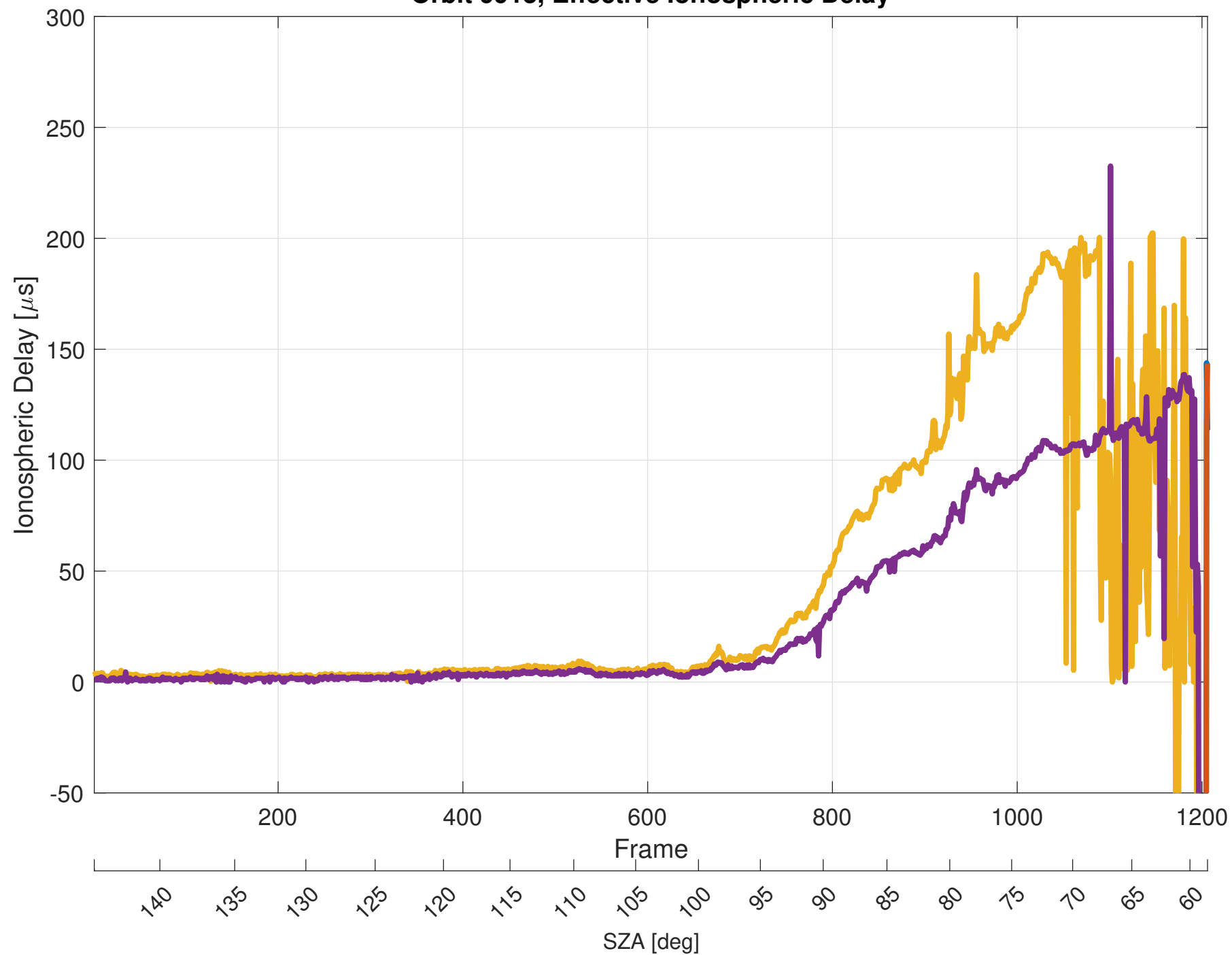
Orbit 9913, Effective Ionospheric Delay
