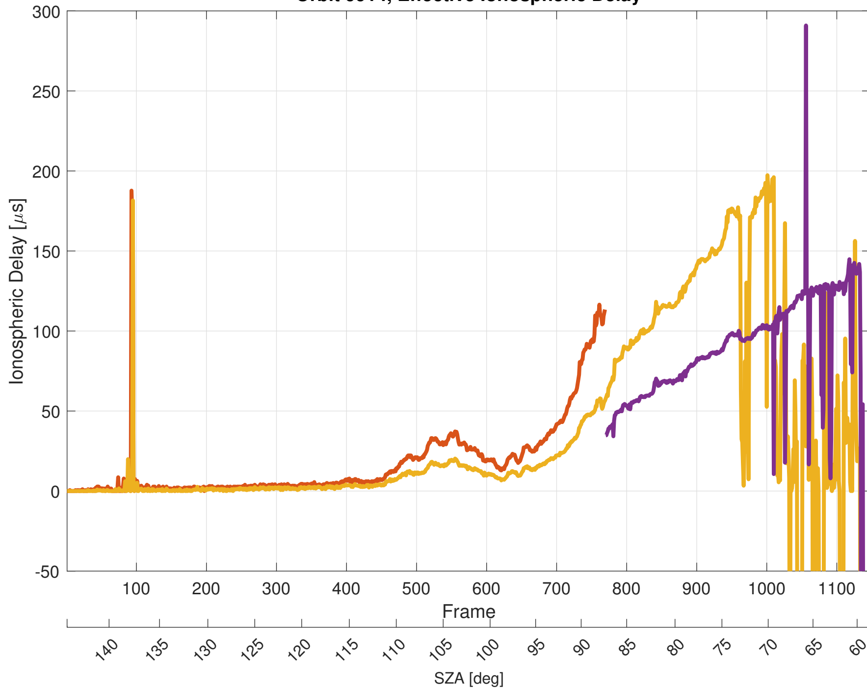
Orbit 9914, Effective Ionospheric Delay
