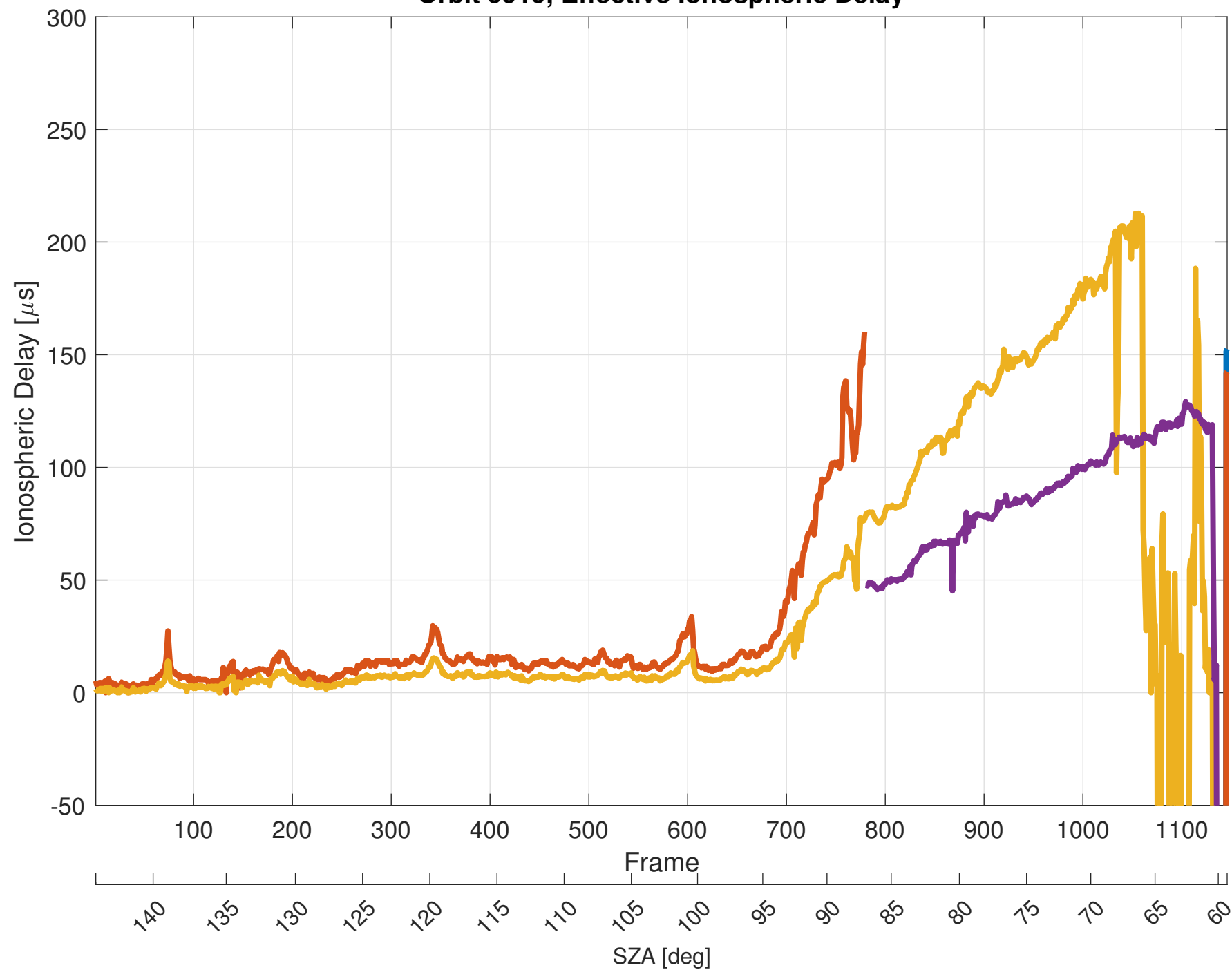
Orbit 9919, Effective Ionospheric Delay
