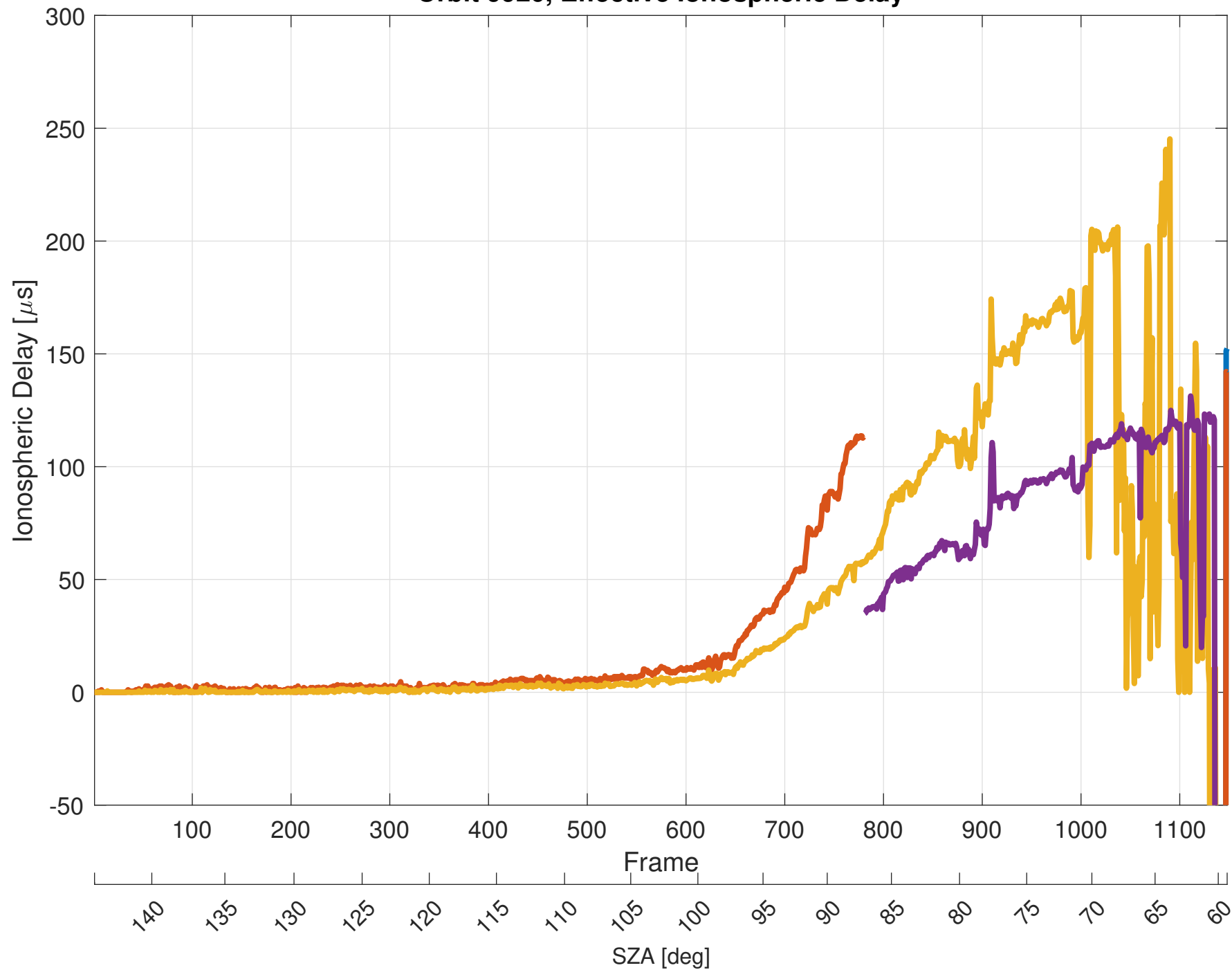
Orbit 9920, Effective Ionospheric Delay
