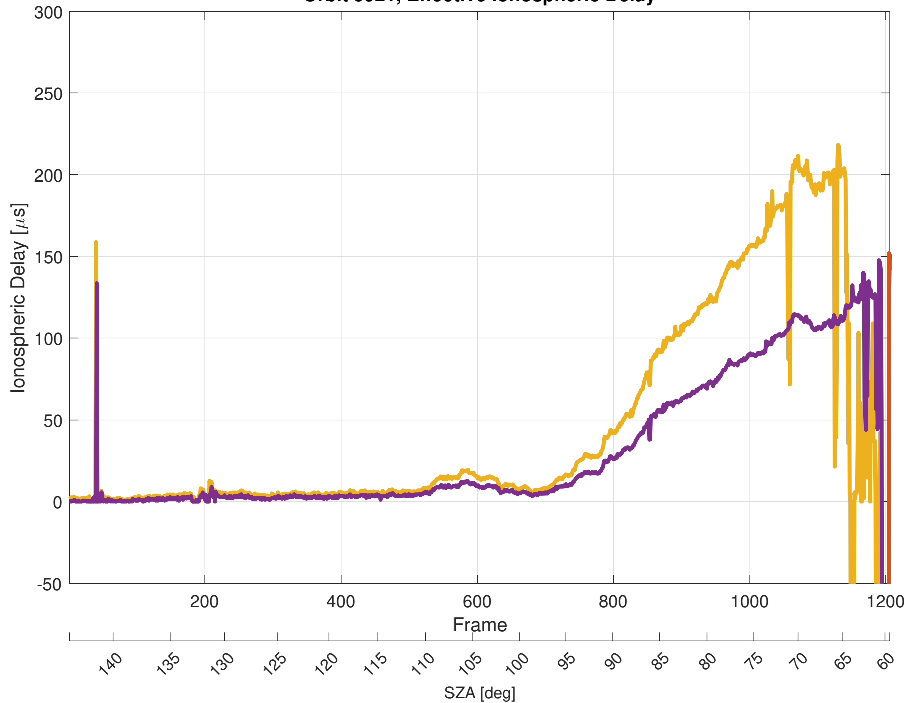
Orbit 9921, Effective Ionospheric Delay
