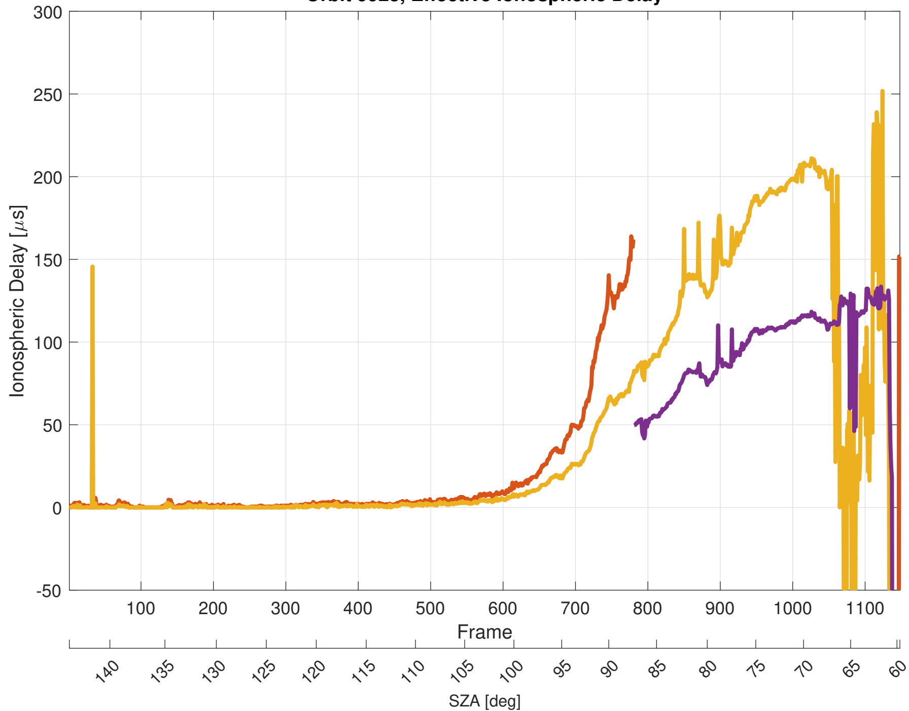
Orbit 9923, Effective Ionospheric Delay
