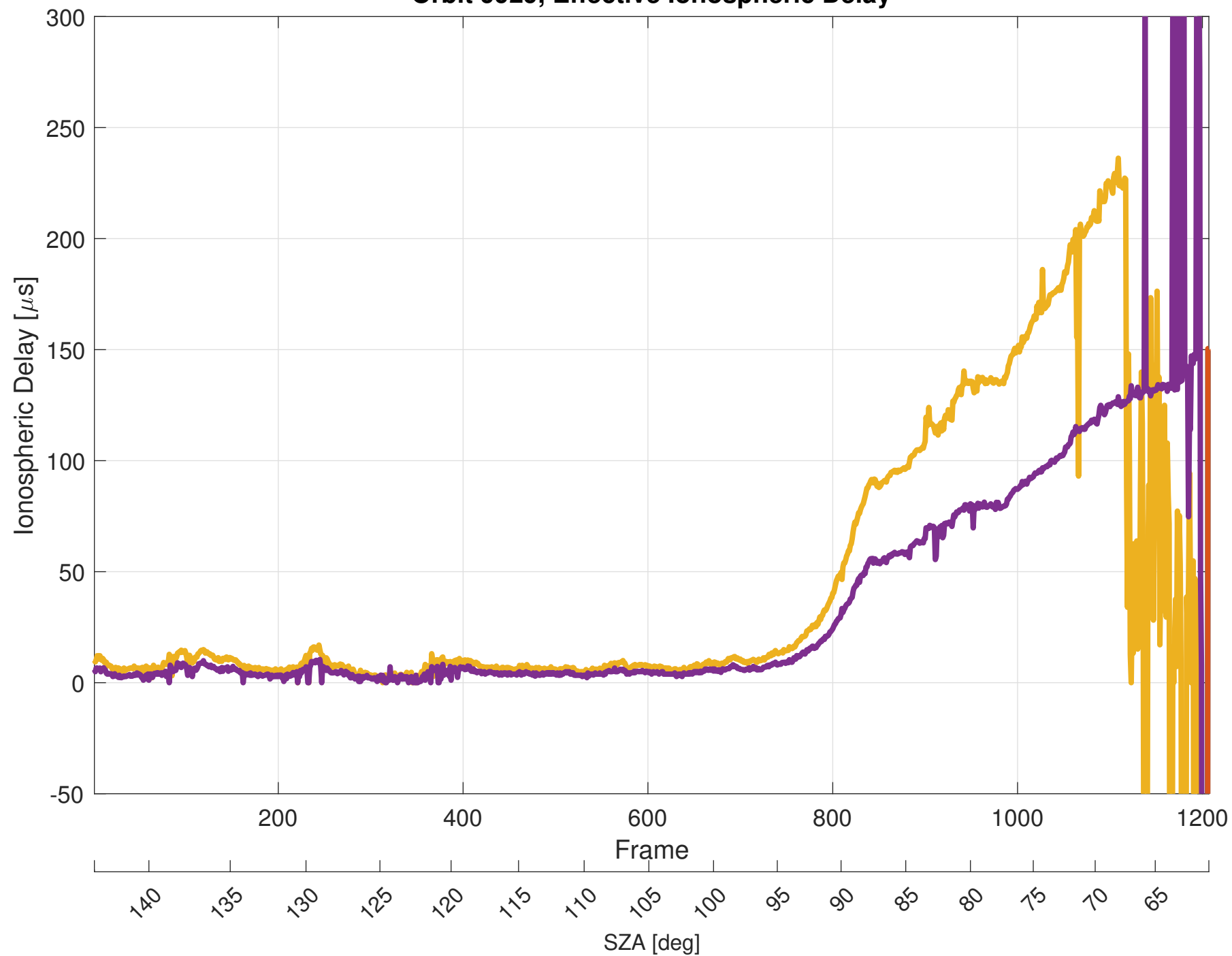
Orbit 9929, Effective Ionospheric Delay
