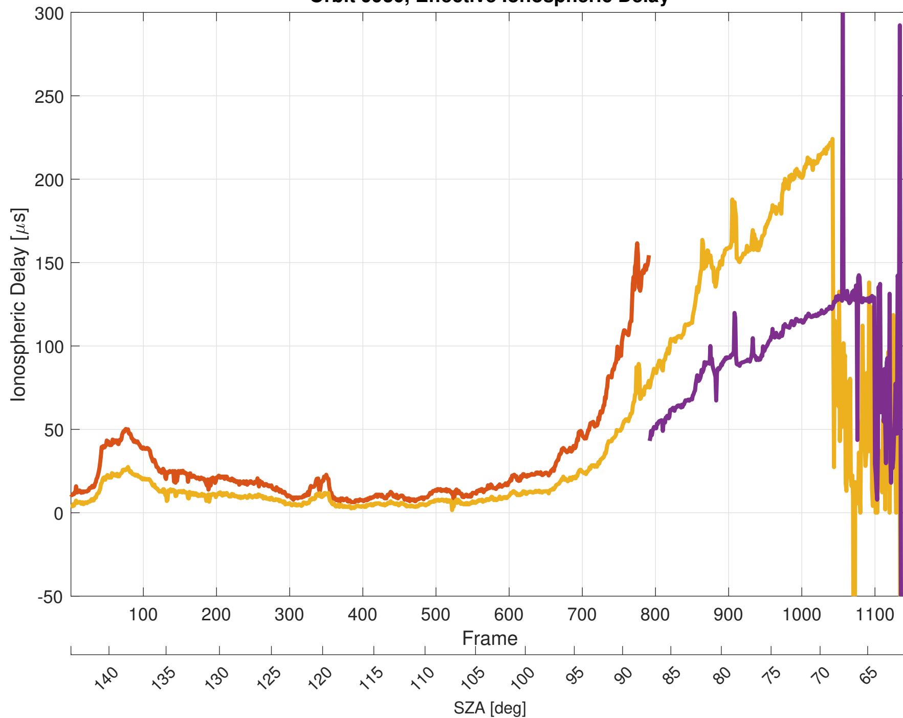
Orbit 9930, Effective Ionospheric Delay
