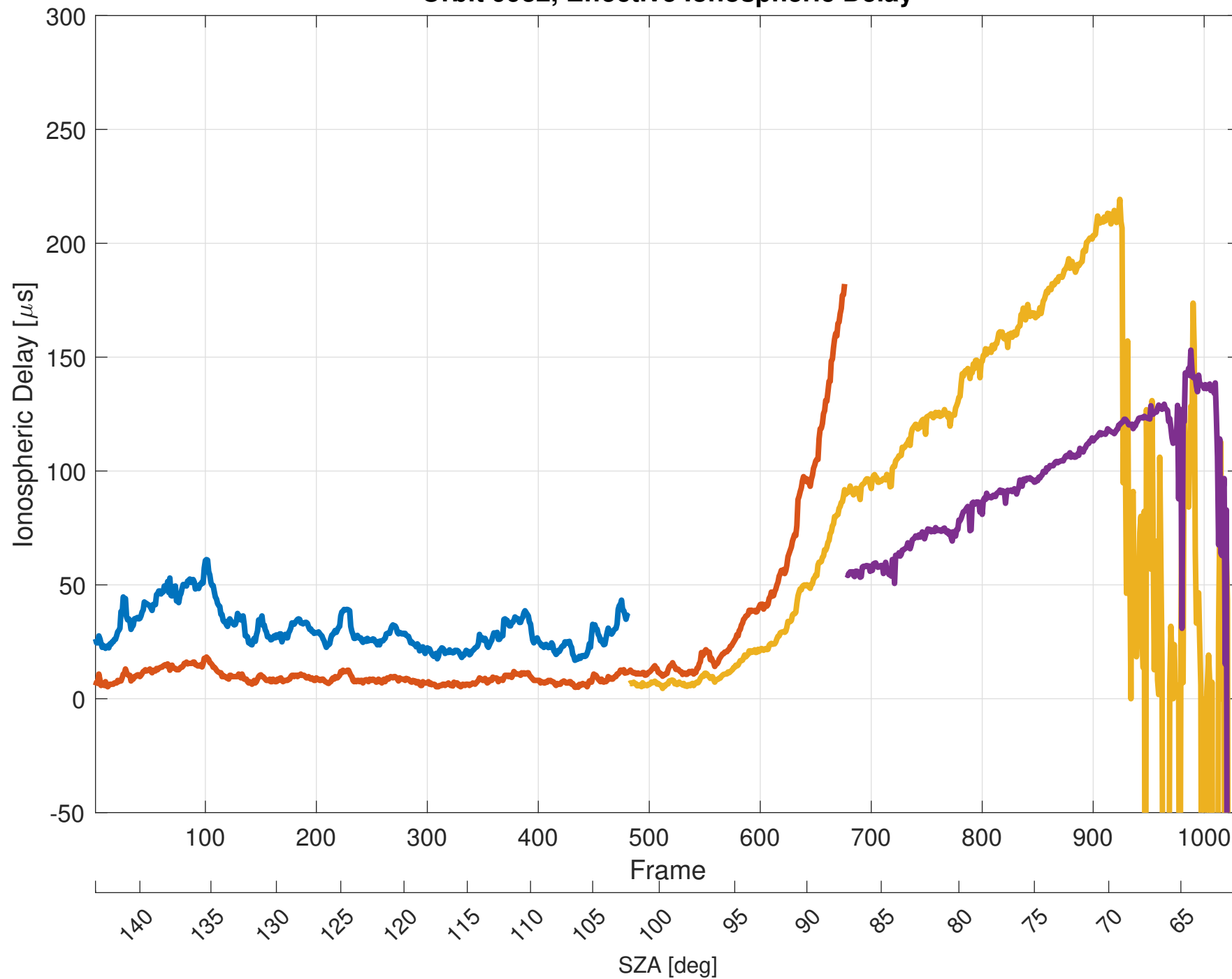
Orbit 9932, Effective Ionospheric Delay
