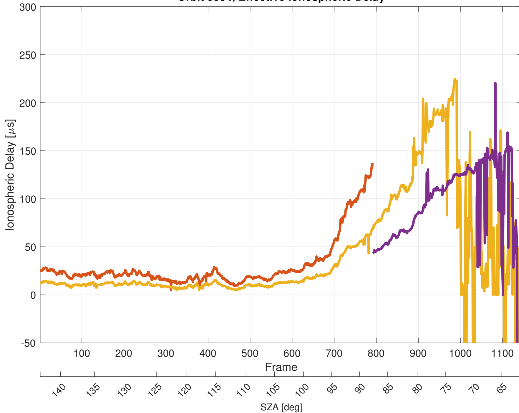
Orbit 9934, Effective Ionospheric Delay
