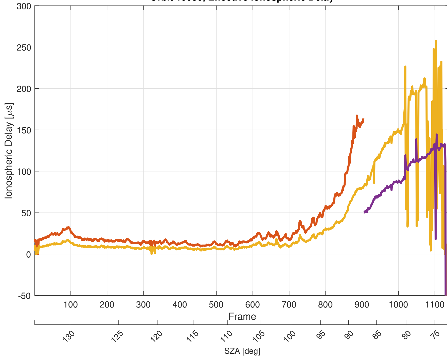
Orbit 10036, Effective Ionospheric Delay
