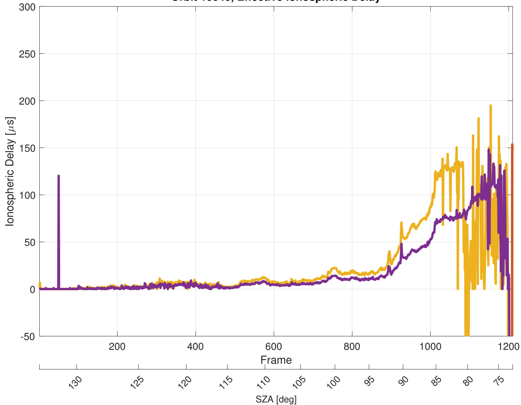
Orbit 10040, Effective Ionospheric Delay
