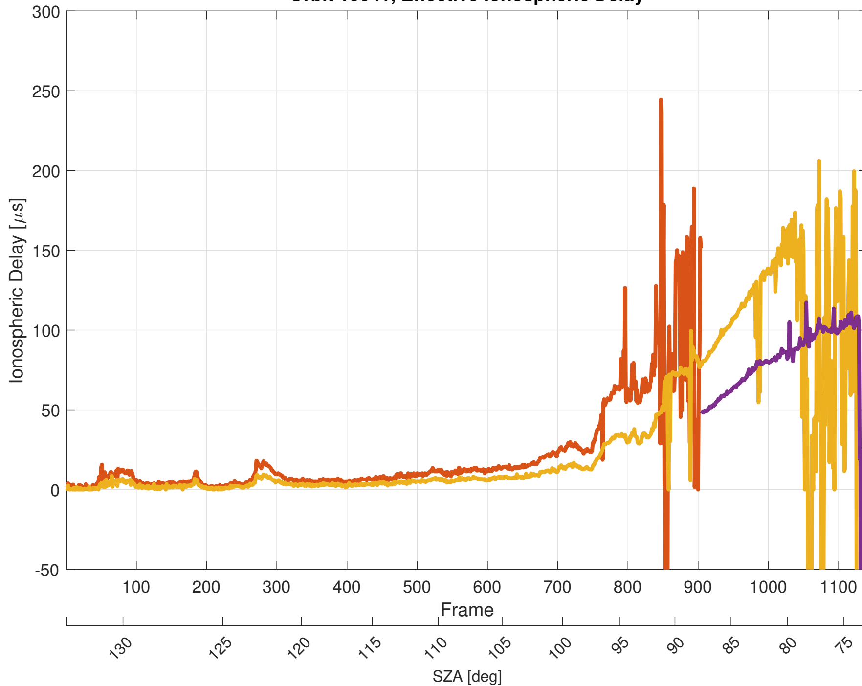
Orbit 10041, Effective Ionospheric Delay
