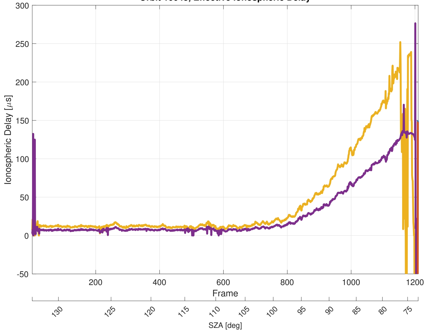
Orbit 10043, Effective Ionospheric Delay
