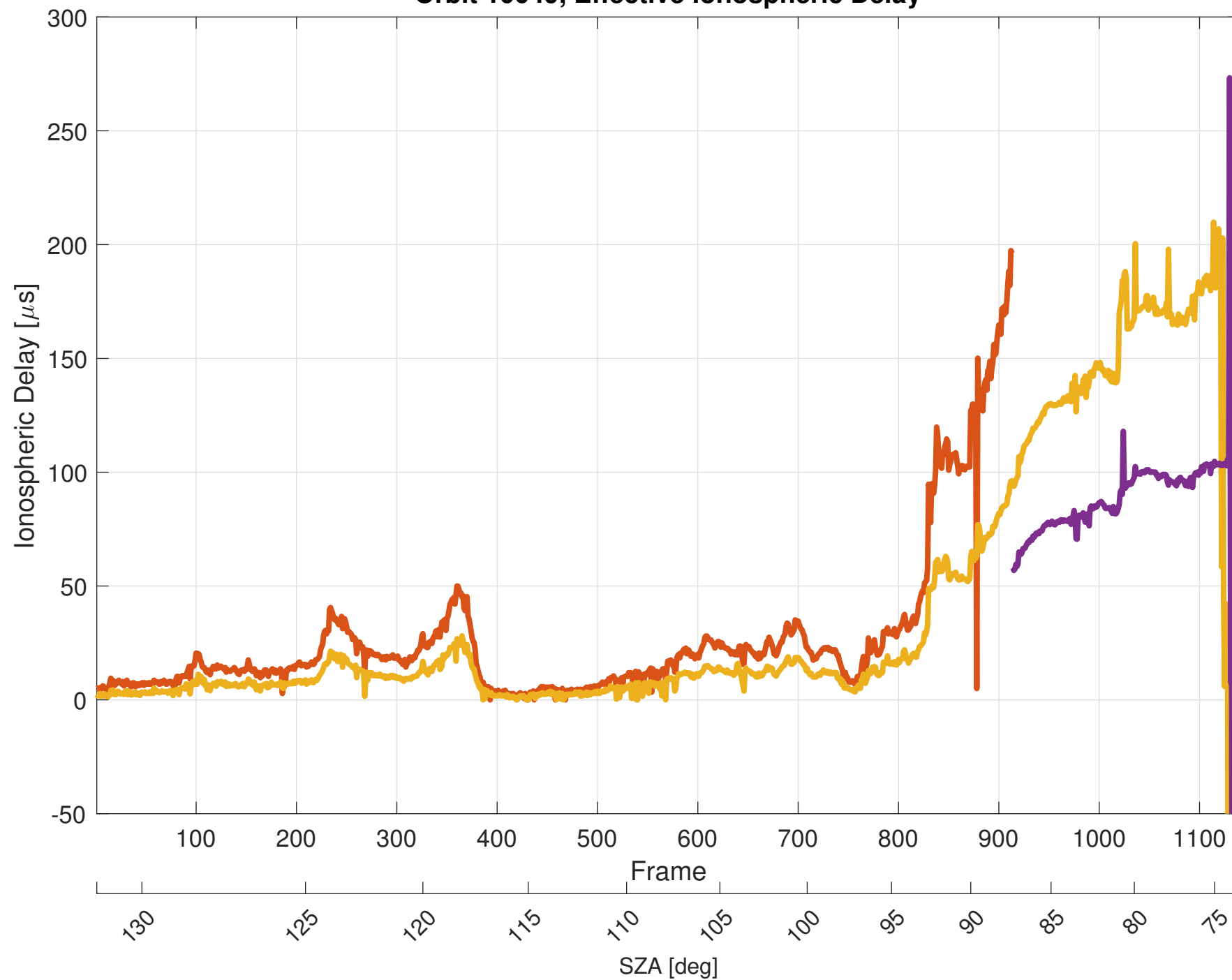
Orbit 10049, Effective Ionospheric Delay
