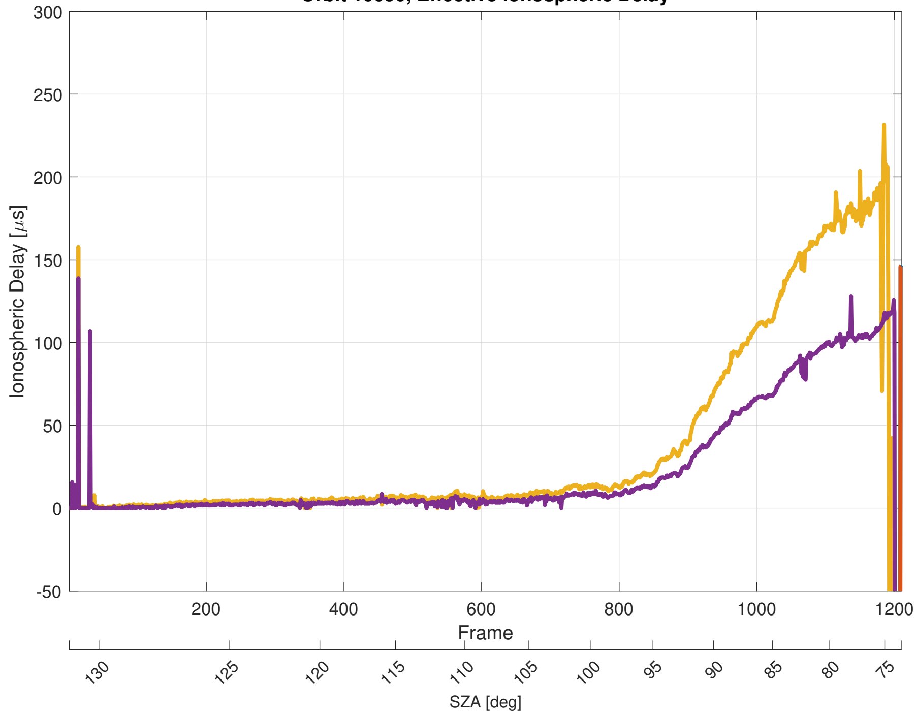
Orbit 10050, Effective Ionospheric Delay
