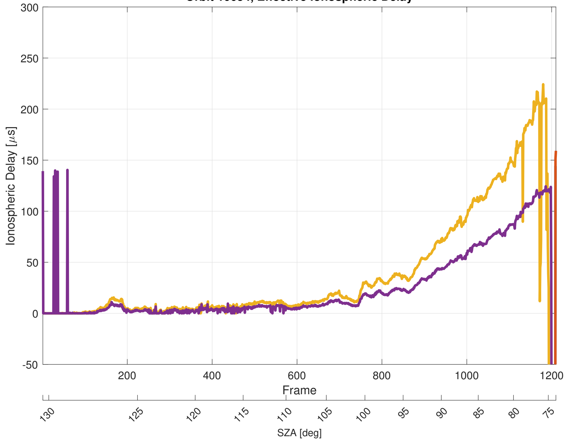
Orbit 10054, Effective Ionospheric Delay
